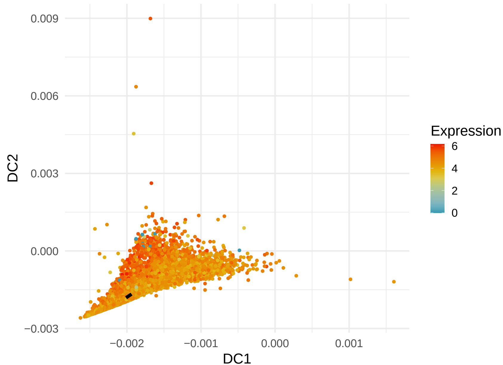
MT-CO2 Expression along Lineage 9 ( R = -0.285 )
