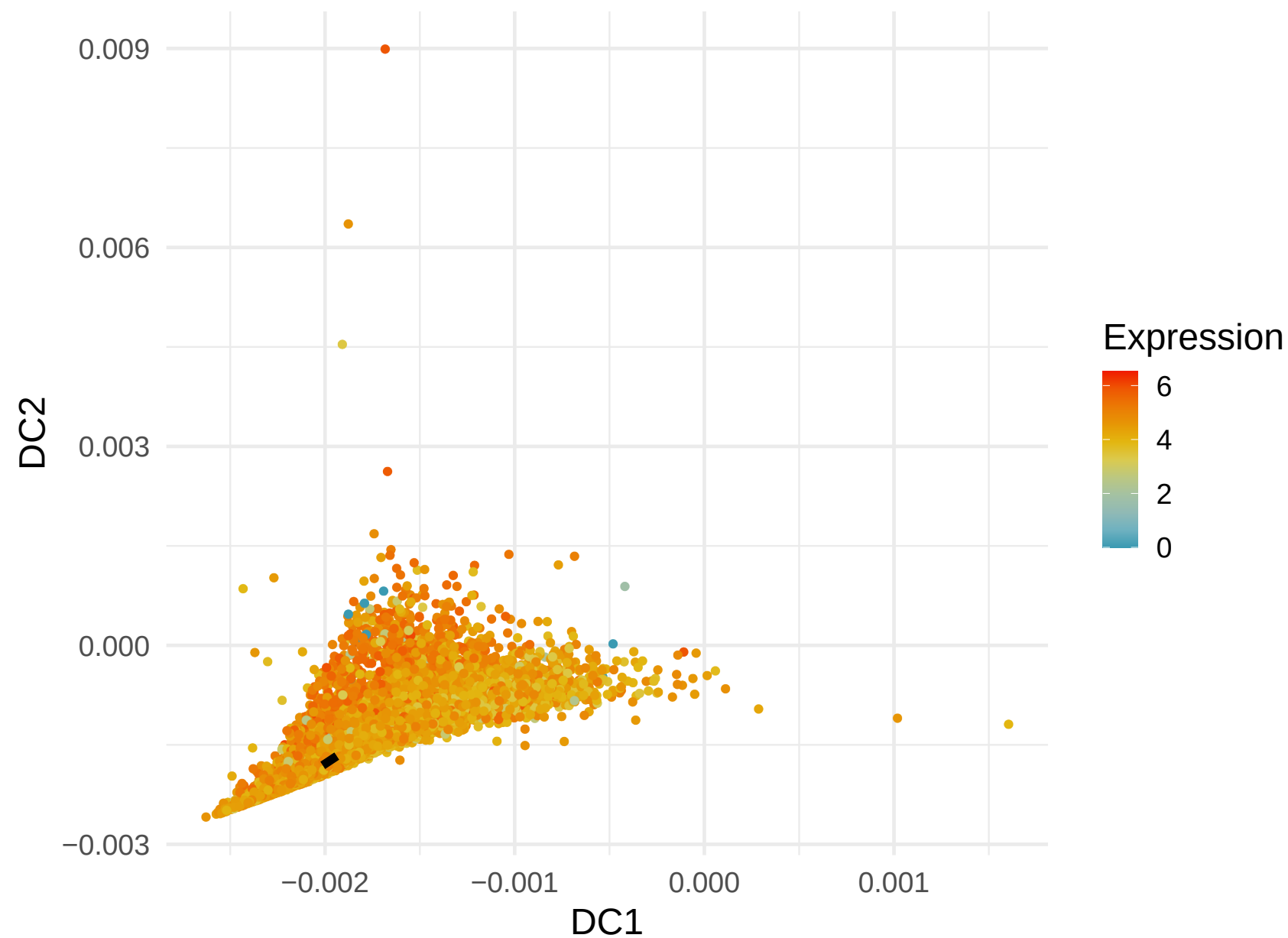
MT-CO3 Expression along Lineage 9 ( R = -0.182 )
