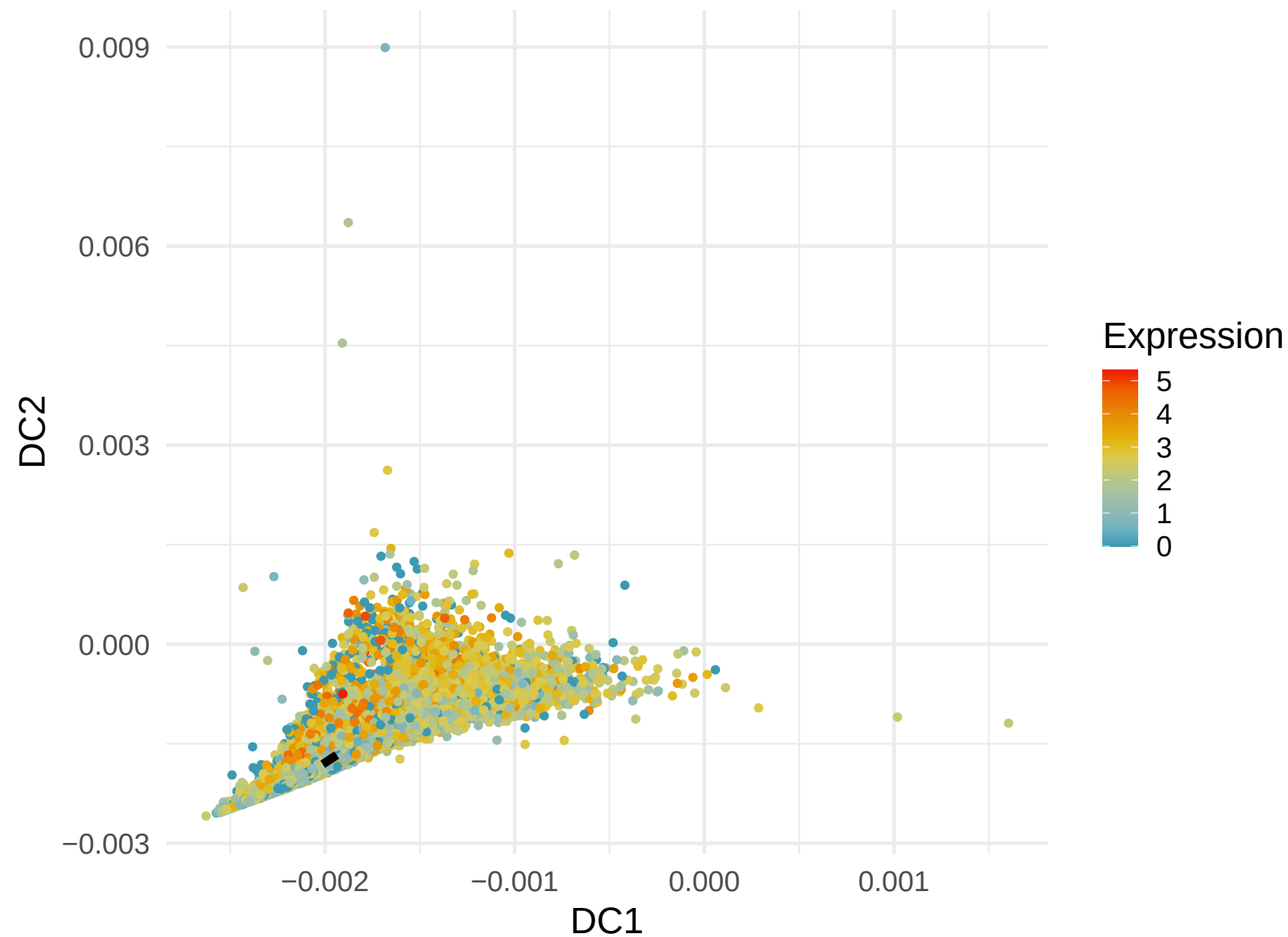
NAMPT Expression along Lineage 9 ( R = -0.22 )
