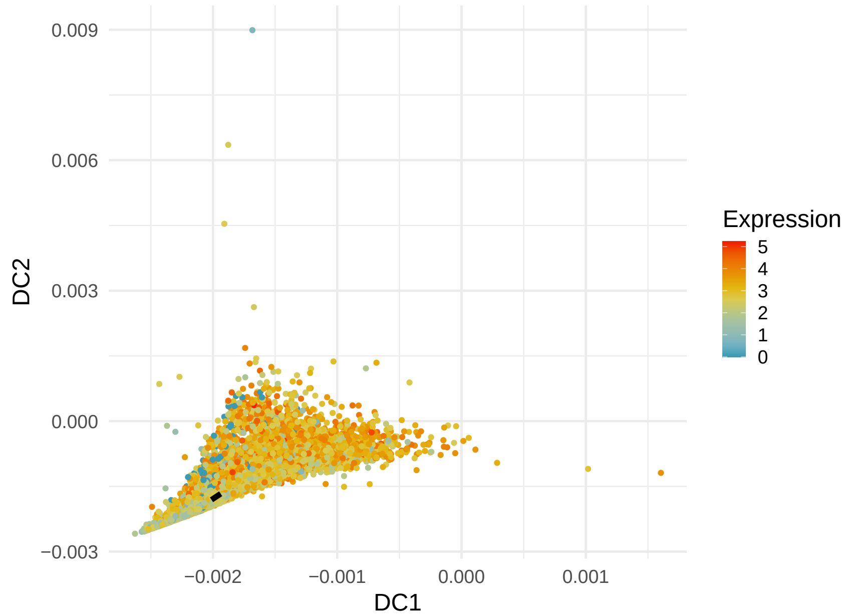
SAT1 Expression along Lineage 9 ( R = -0.18 )
