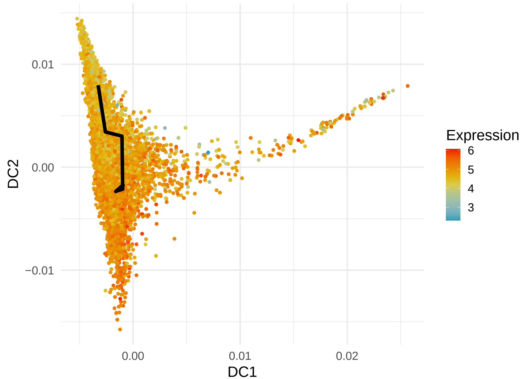
B2M Expression along Lineage 1 ( R = 0.381 )
