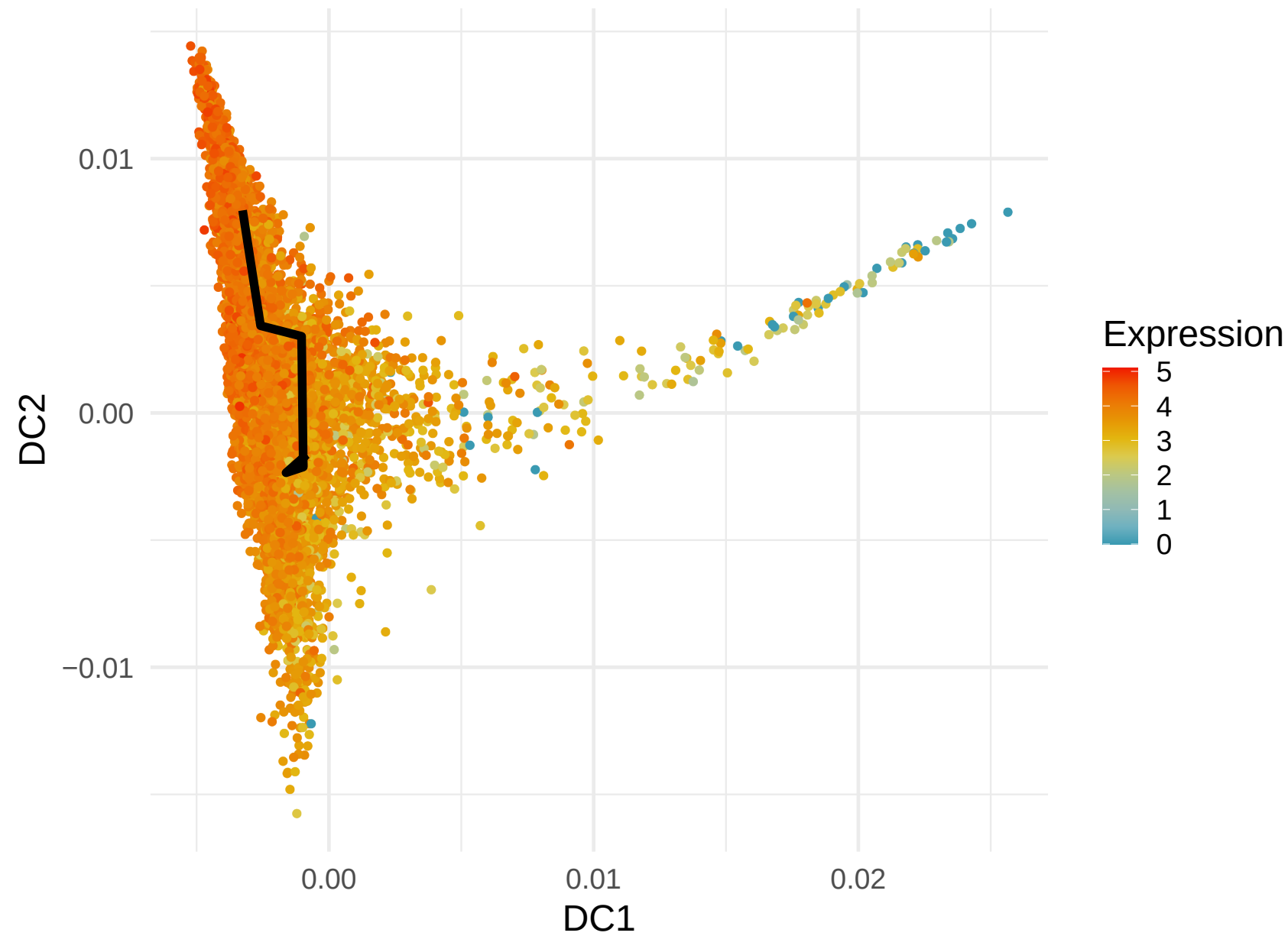
RPS23 Expression along Lineage 1 ( R = -0.288 )
