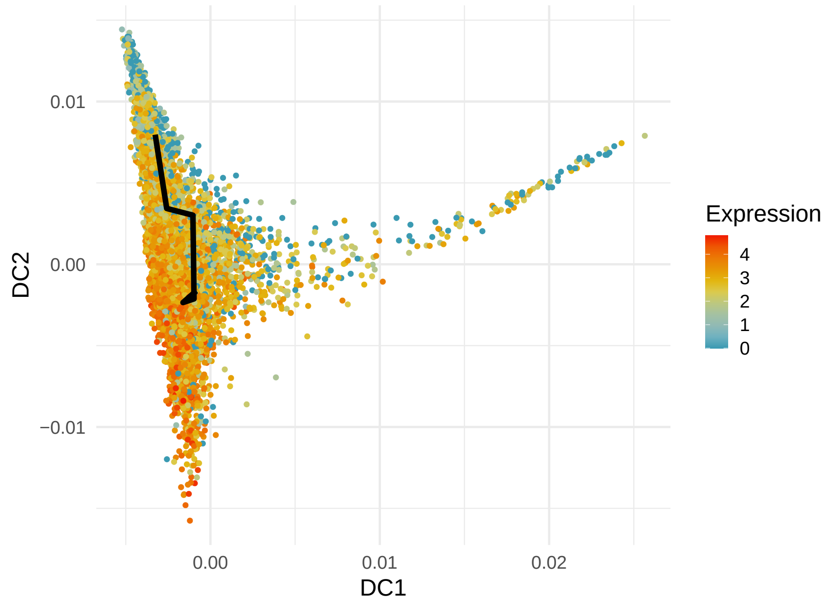
S100A4 Expression along Lineage 1 ( R = 0.472 )
