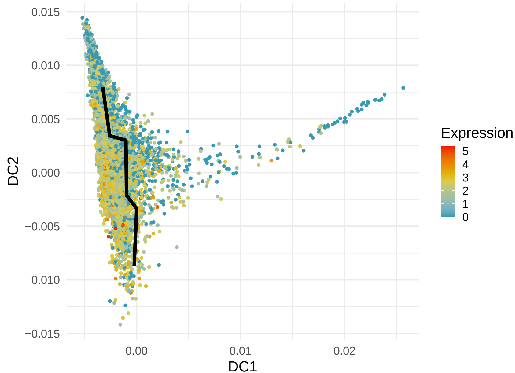
CRIP1 Expression along Lineage 2 ( R = 0.263 )
