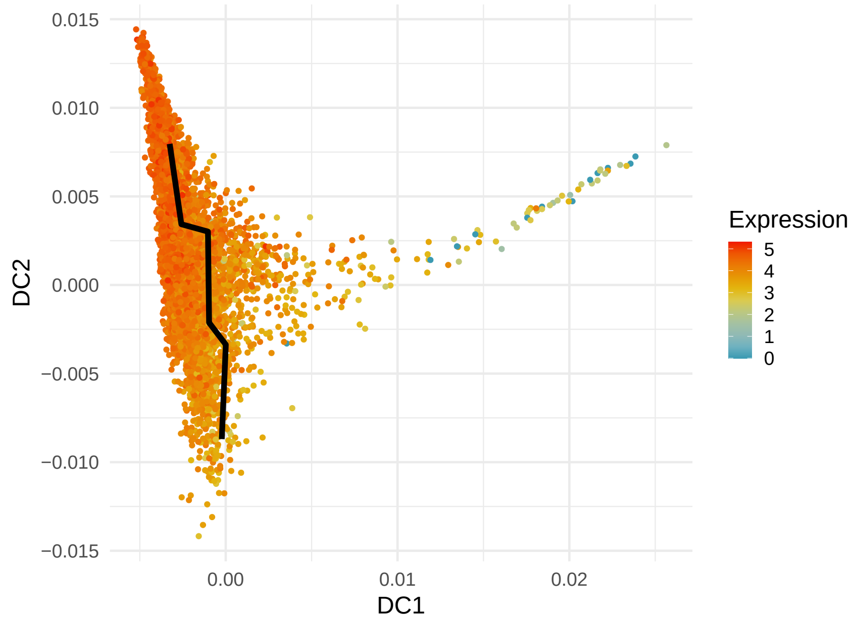
RPL34 Expression along Lineage 2 ( R = -0.365 )
