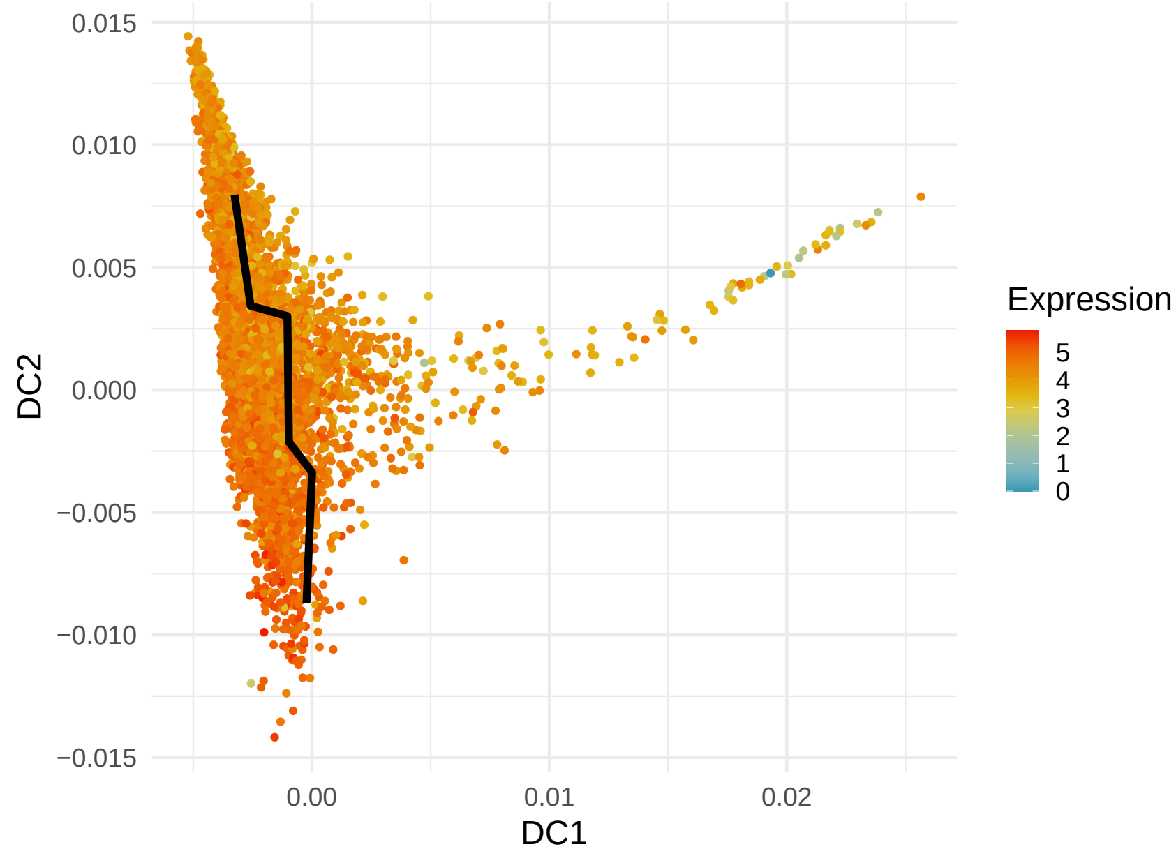
TMSB4X Expression along Lineage 2 ( R = 0.283 )
