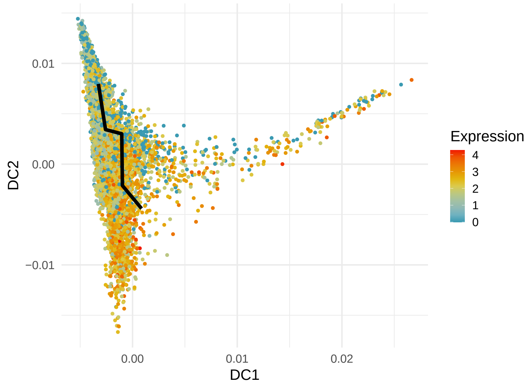
CD2 Expression along Lineage 3 ( R = 0.377 )
