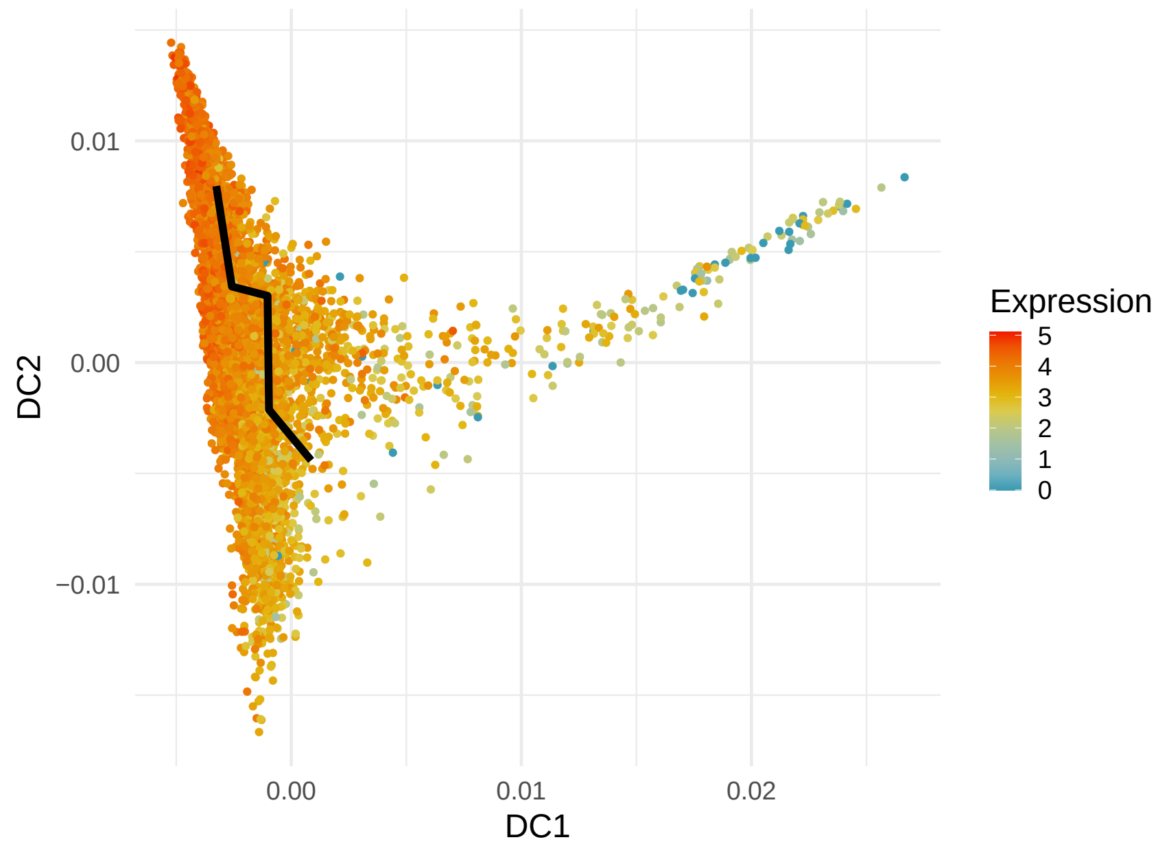
RPS8 Expression along Lineage 3 ( R = -0.379 )
