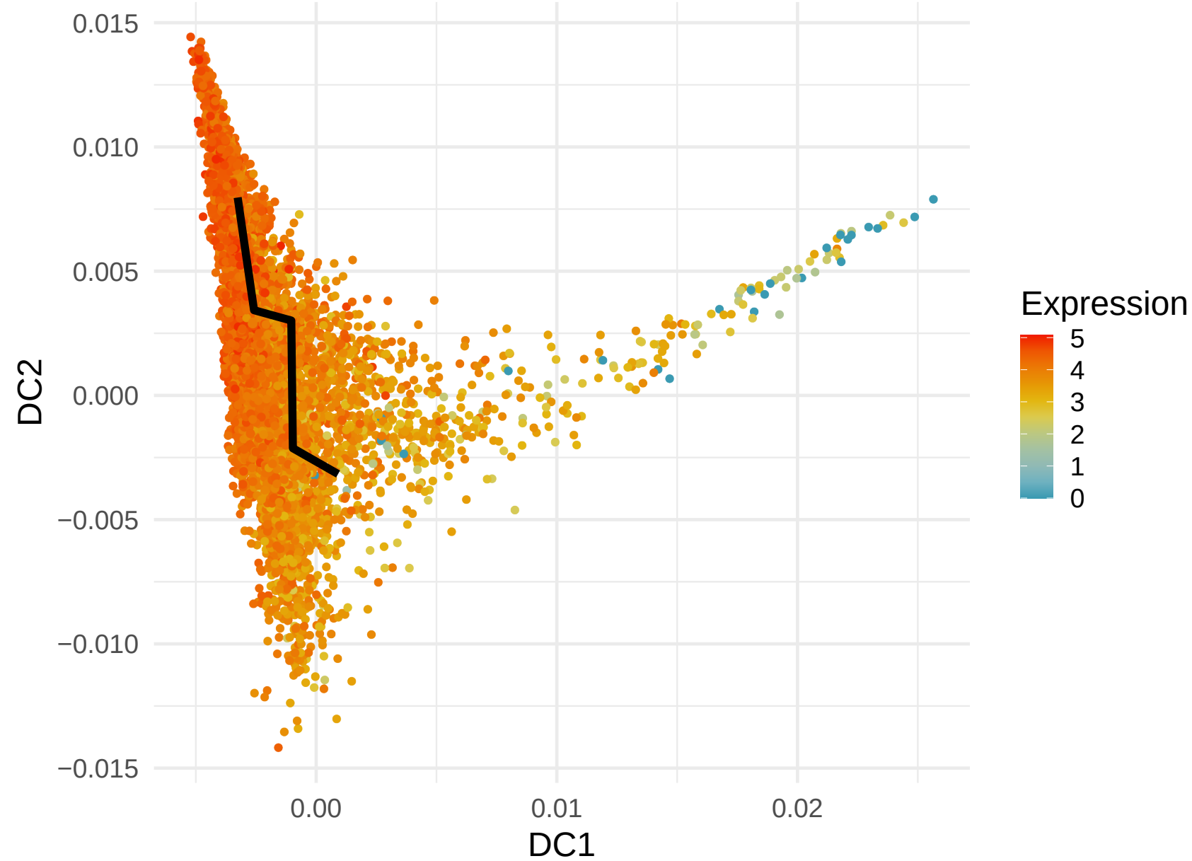
RPL37 Expression along Lineage 4 ( R = -0.441 )
