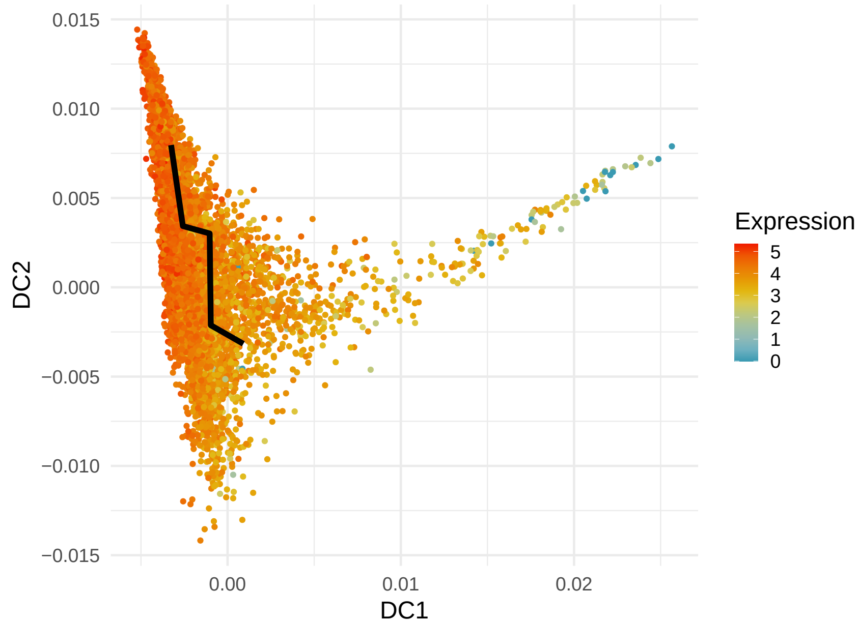
RPS18 Expression along Lineage 4 ( R = -0.427 )
