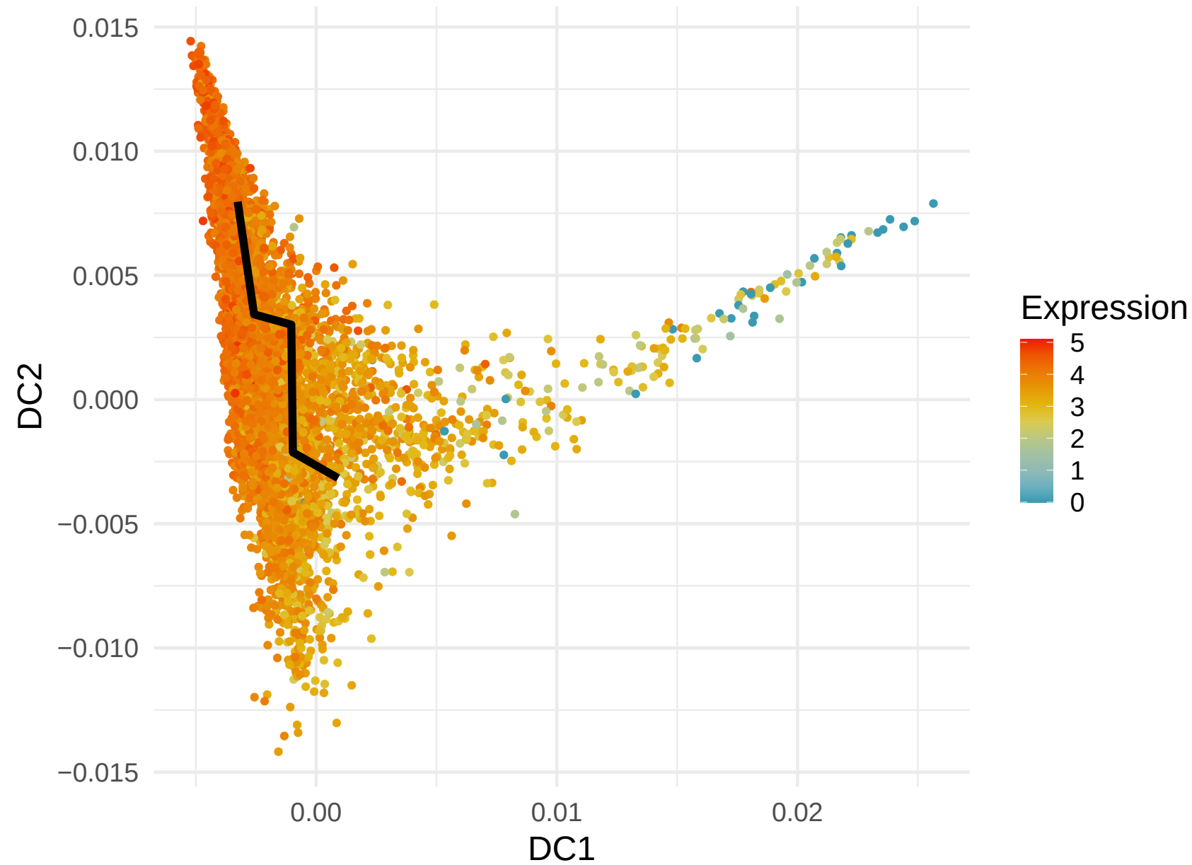
RPS23 Expression along Lineage 4 ( R = -0.434 )
