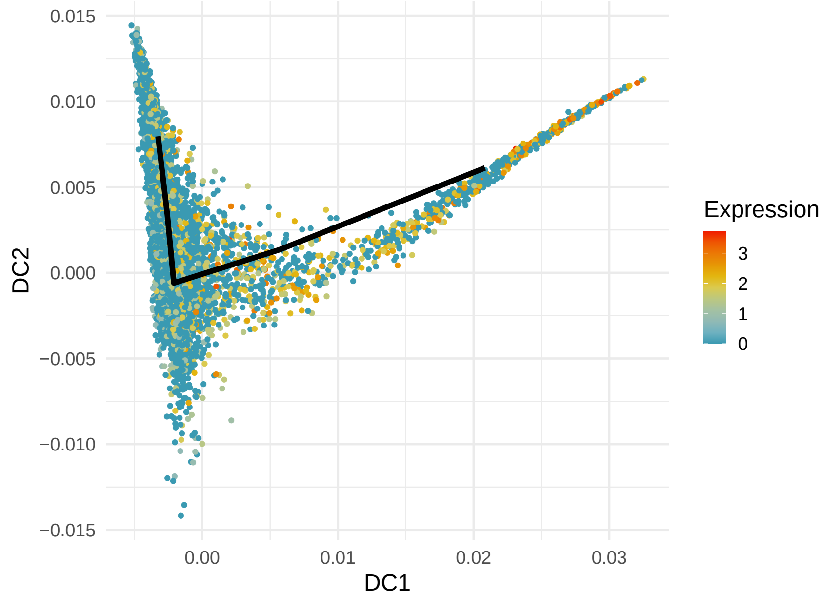
AC004687.1 Expression along Lineage 5 ( R = 0.221 )
