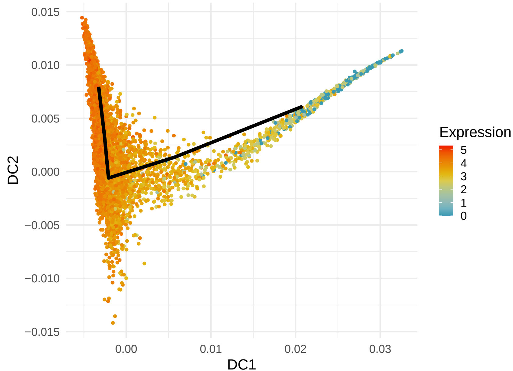
RPL11 Expression along Lineage 5 ( R = -0.7 )
