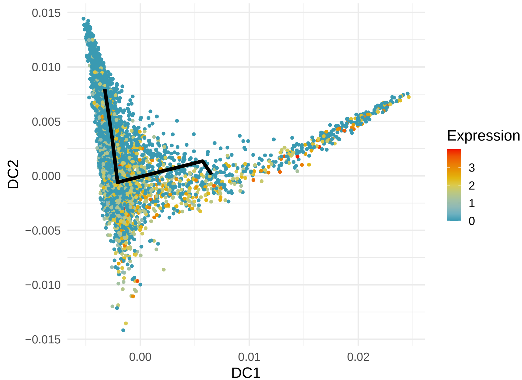
MAF Expression along Lineage 6 ( R = 0.259 )
