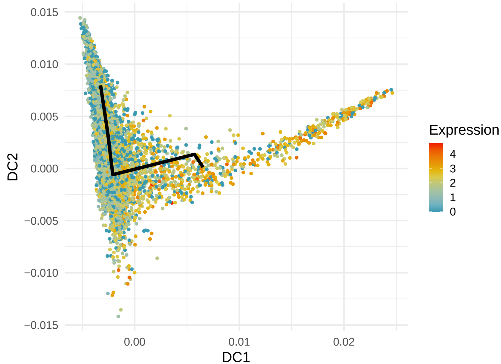
NEAT1 Expression along Lineage 6 (R= 0.213)
