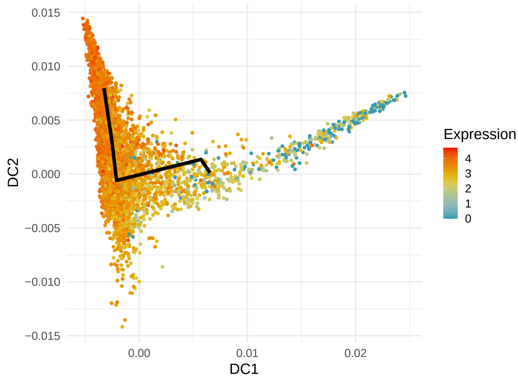
RPS13 Expression along Lineage 6 ( R = -0.456 )
