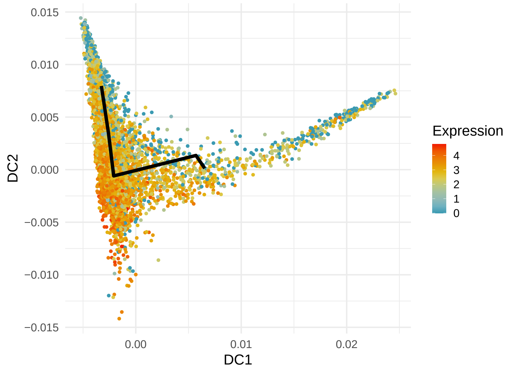
S100A4 Expression along Lineage 6 ( R = 0.277 )
