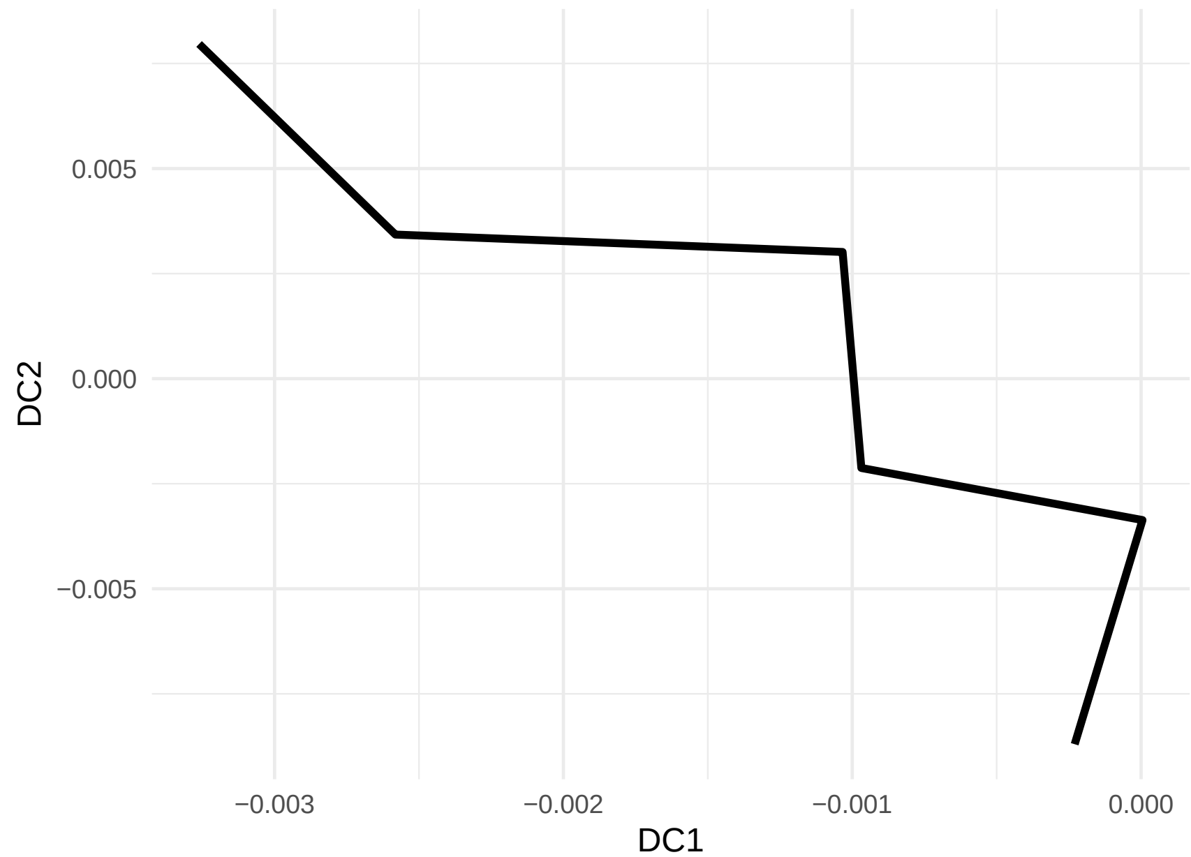
AC023491.2 Expression along Lineage 2 (R= NA)
