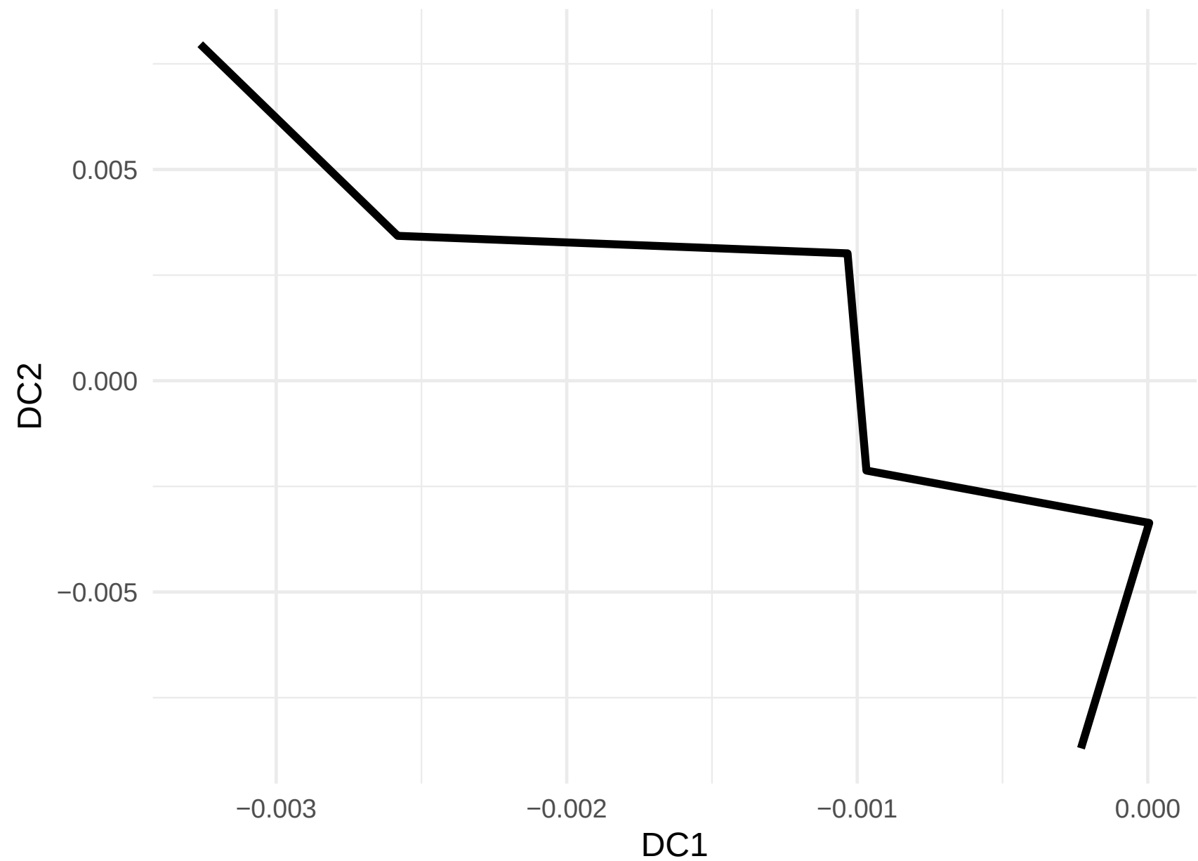
AL627309.2 Expression along Lineage 2 (R= NA)
