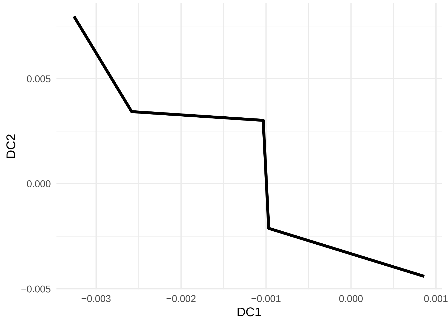
AC141272.1 Expression along Lineage 3 (R= NA)
