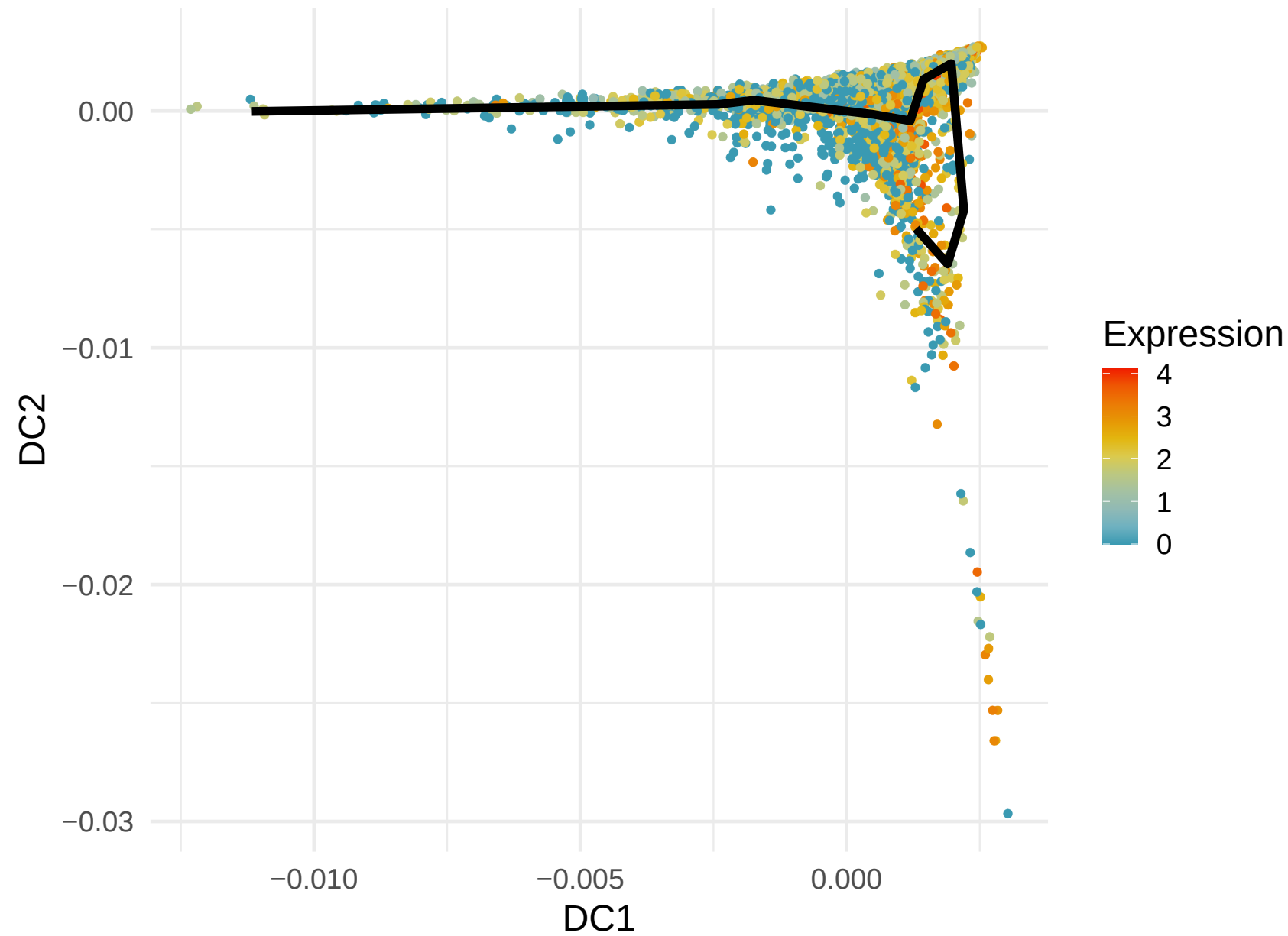
CD74 Expression along Lineage 1 ( R = 0.264 )
