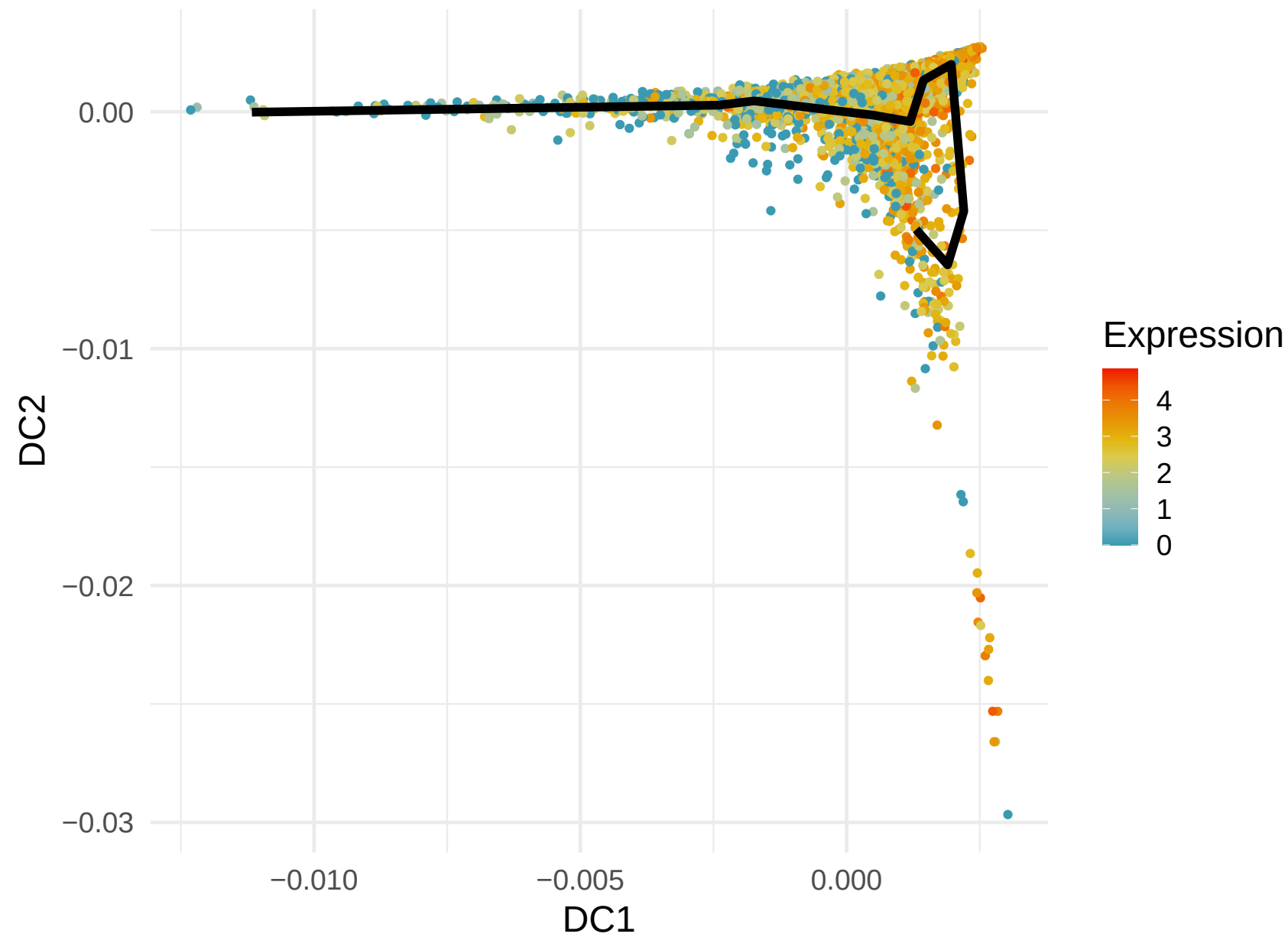
GZMA Expression along Lineage 1 (R= 0.364)
