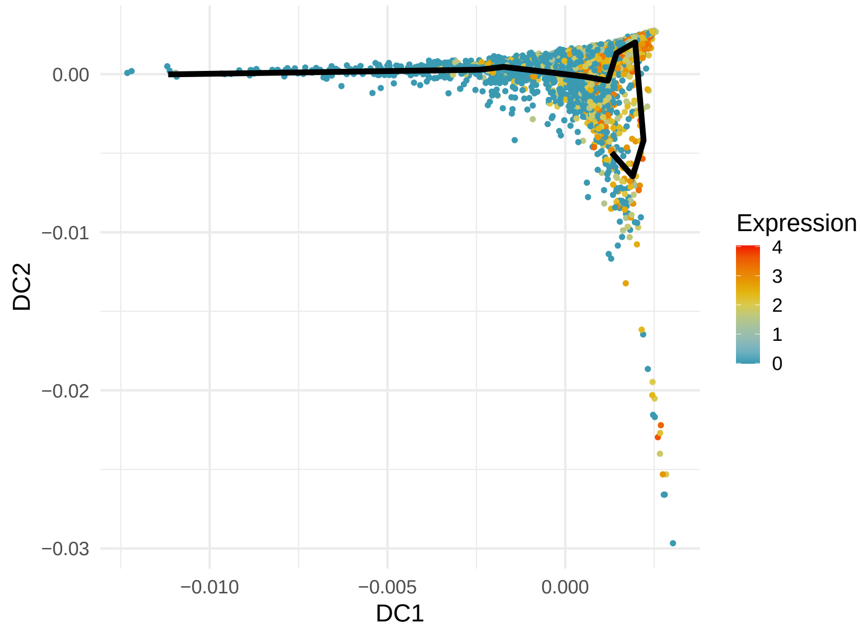
GZMH Expression along Lineage 1 ( R = 0.341 )
