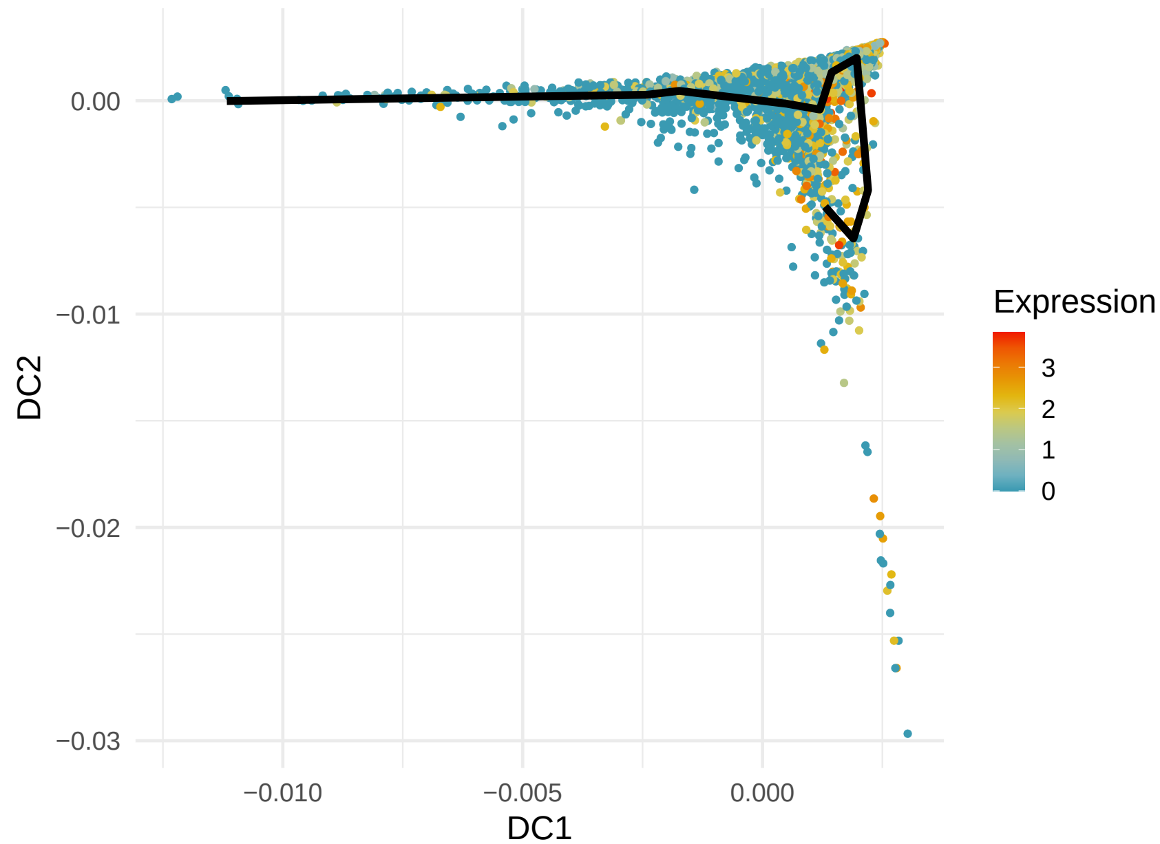
HLA-DRB1 Expression along Lineage 1 ( R = 0.291 )
