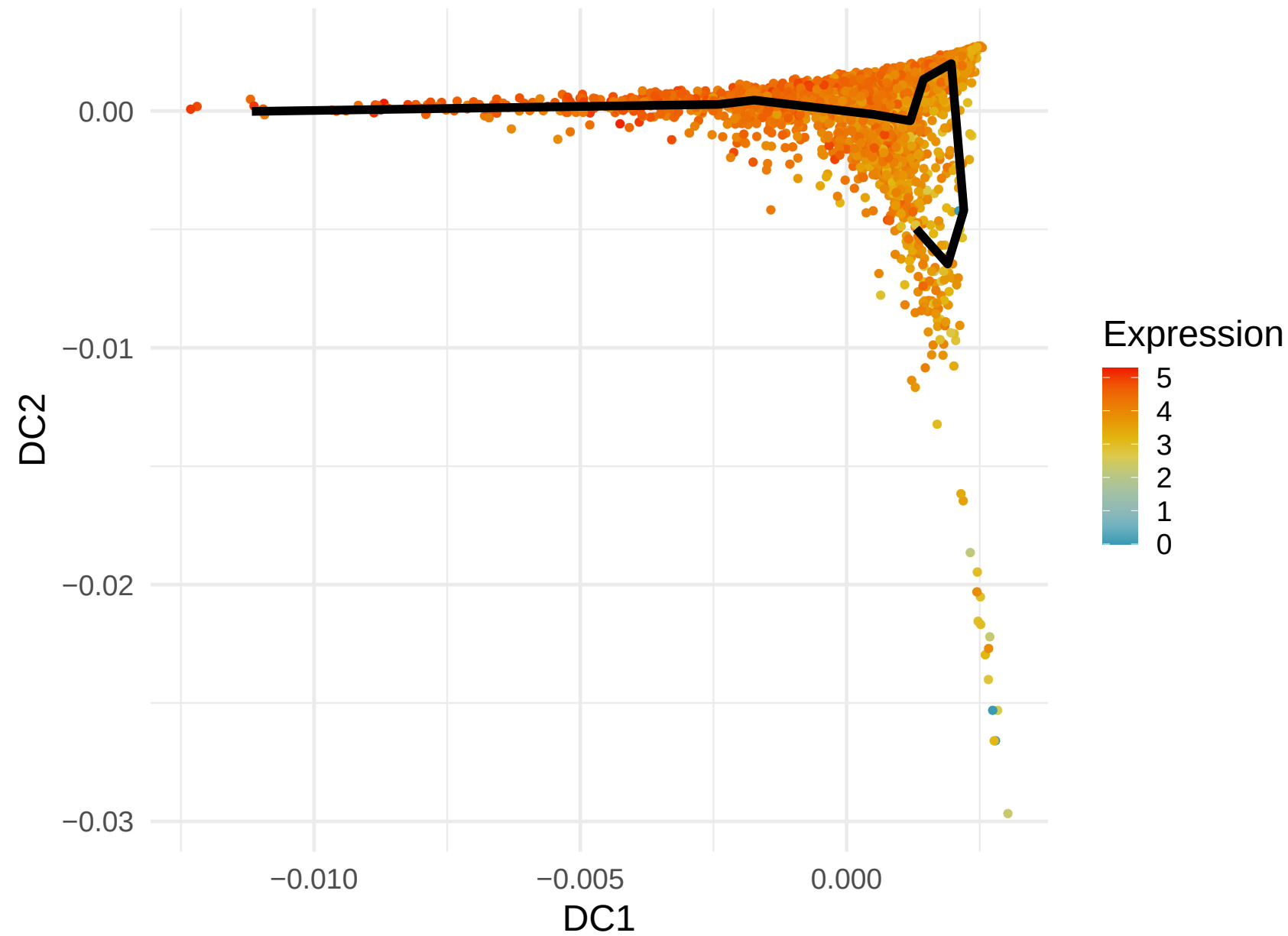
RPL13 Expression along Lineage 1 ( R = -0.351 )
