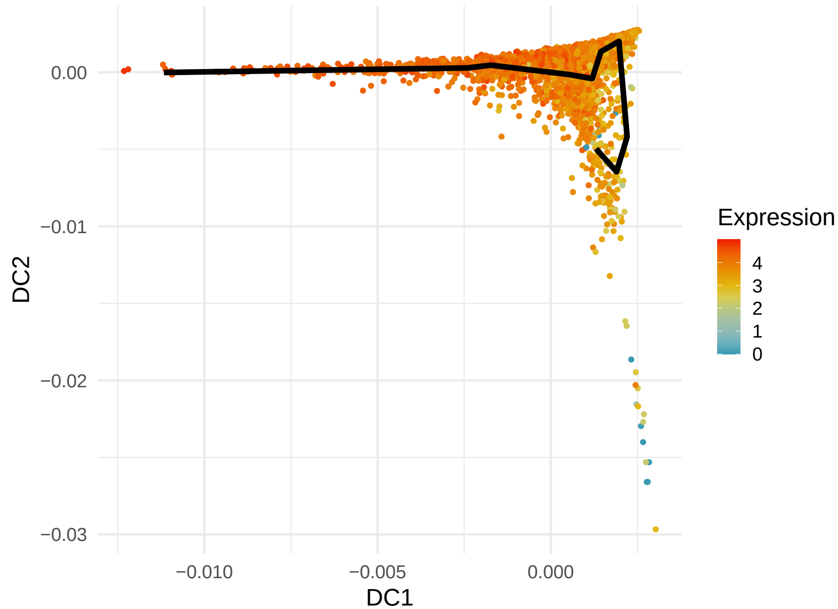
RPL30 Expression along Lineage 1 ( R = -0.327 )
