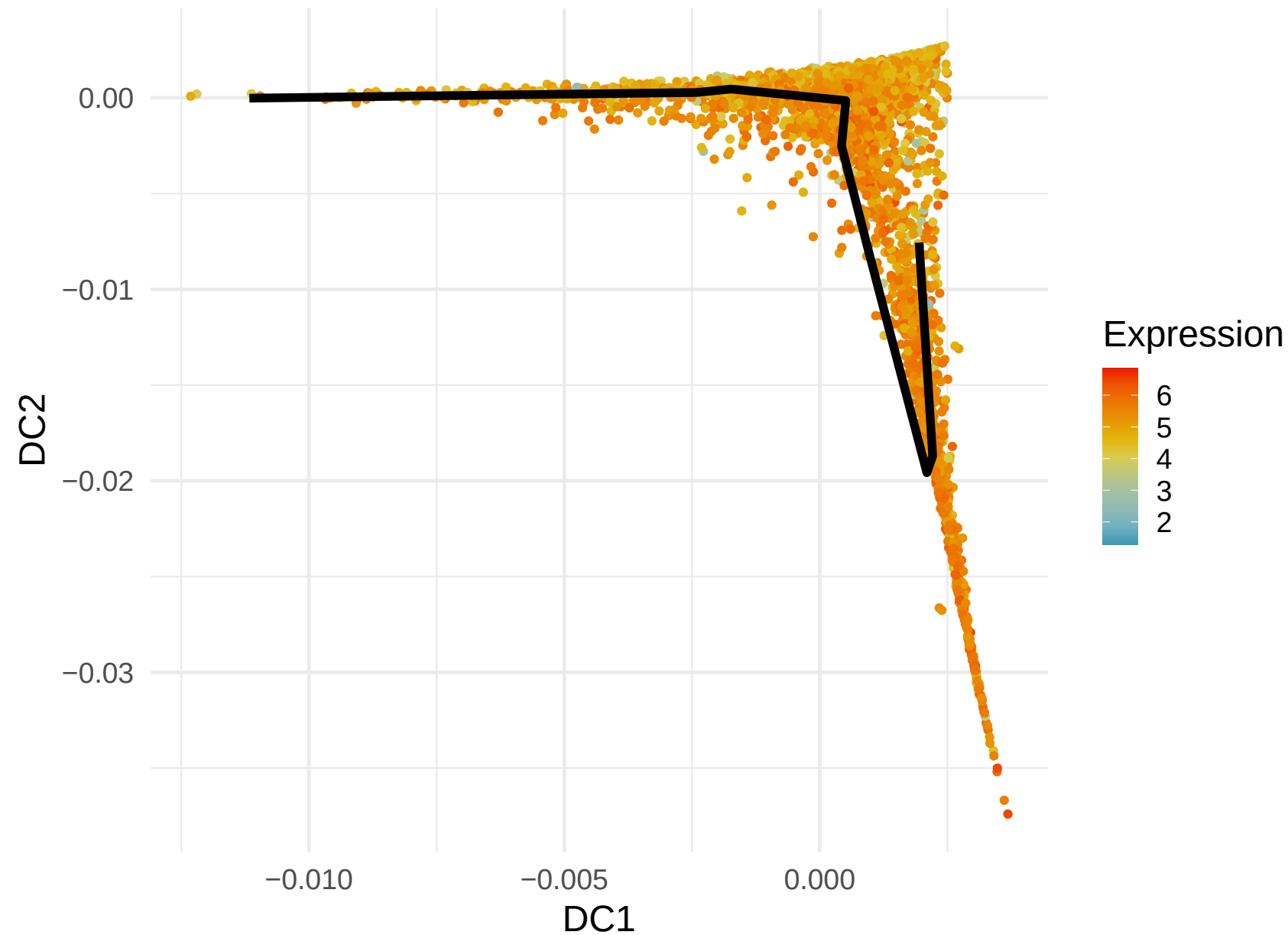
MT-CO1 Expression along Lineage 2 ( R = 0.197 )
