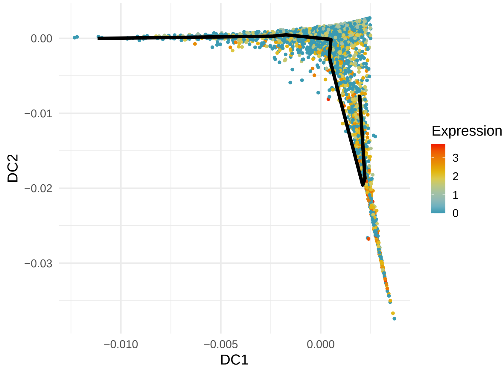
NKTR Expression along Lineage 2 ( R = 0.218 )
