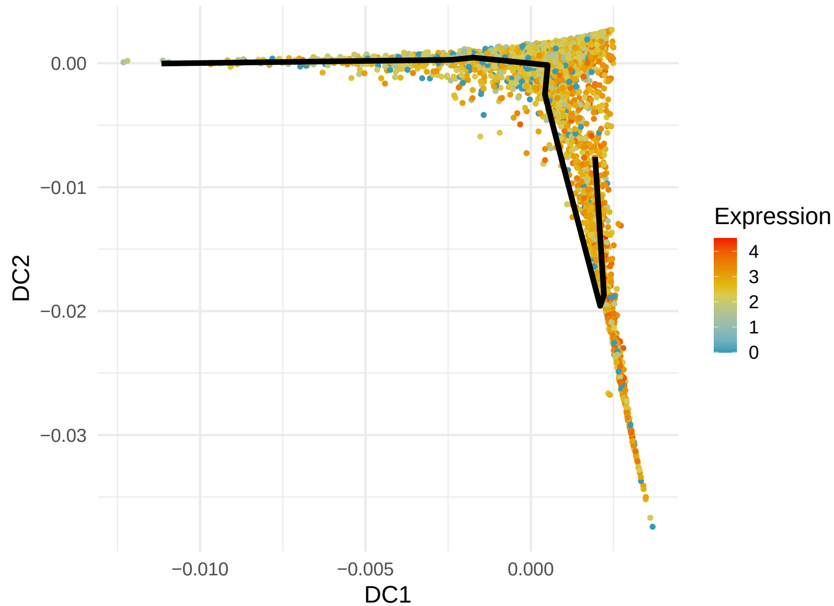
PTPRC Expression along Lineage 2 (R= 0.211)
