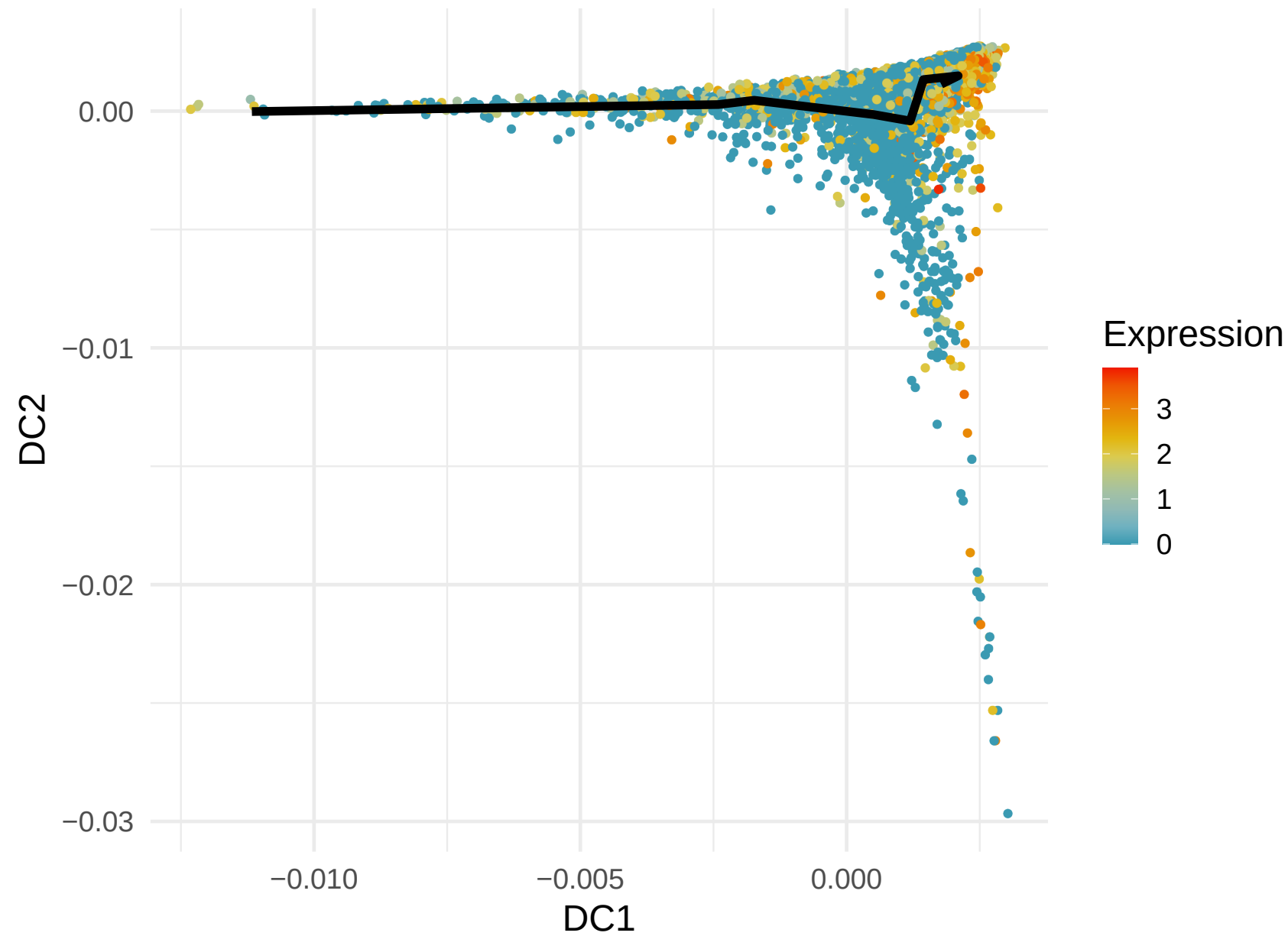
KLF2 Expression along Lineage 3 ( R = 0.541 )
