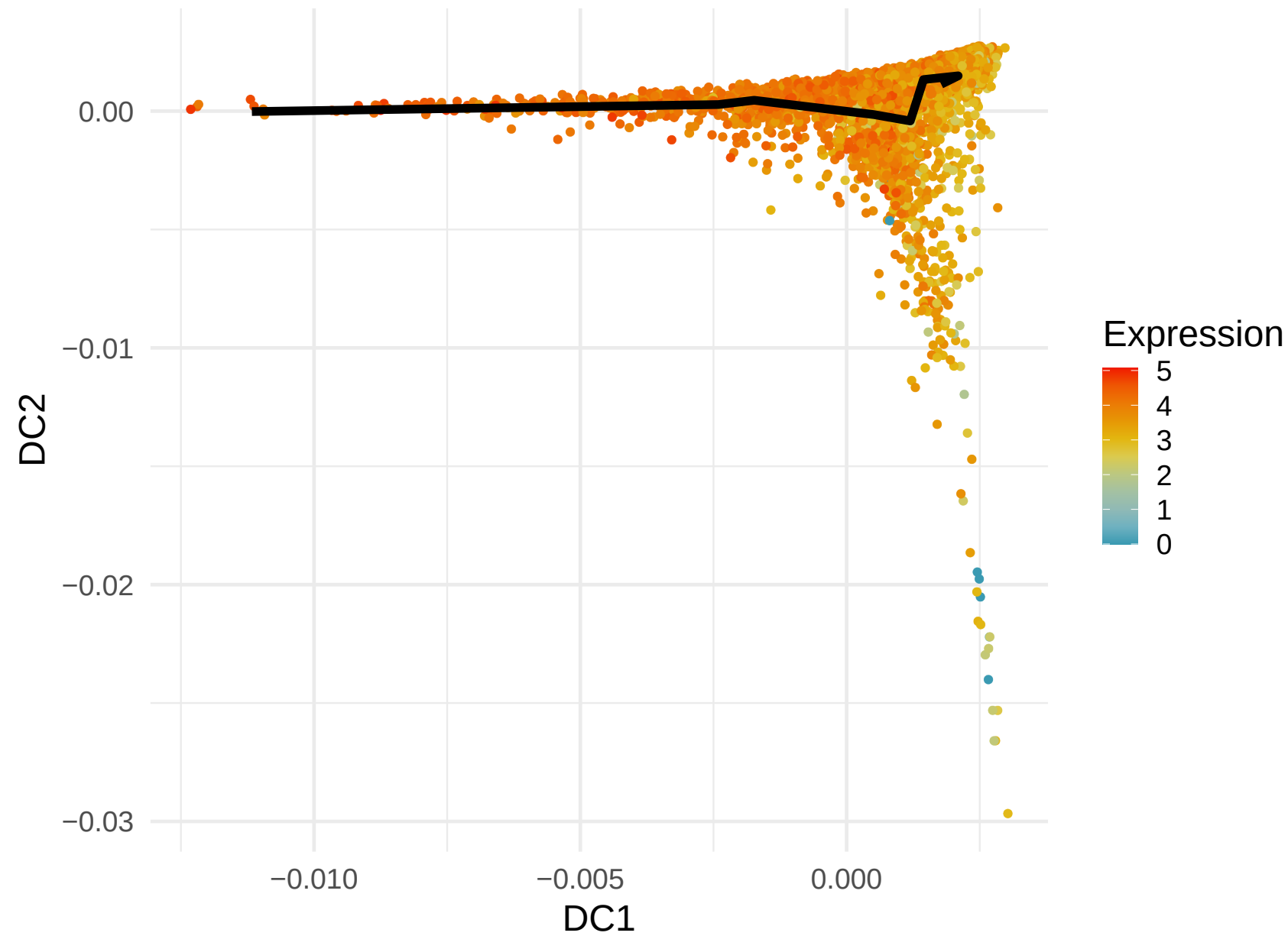
RPS28 Expression along Lineage 3 ( R = -0.259 )
