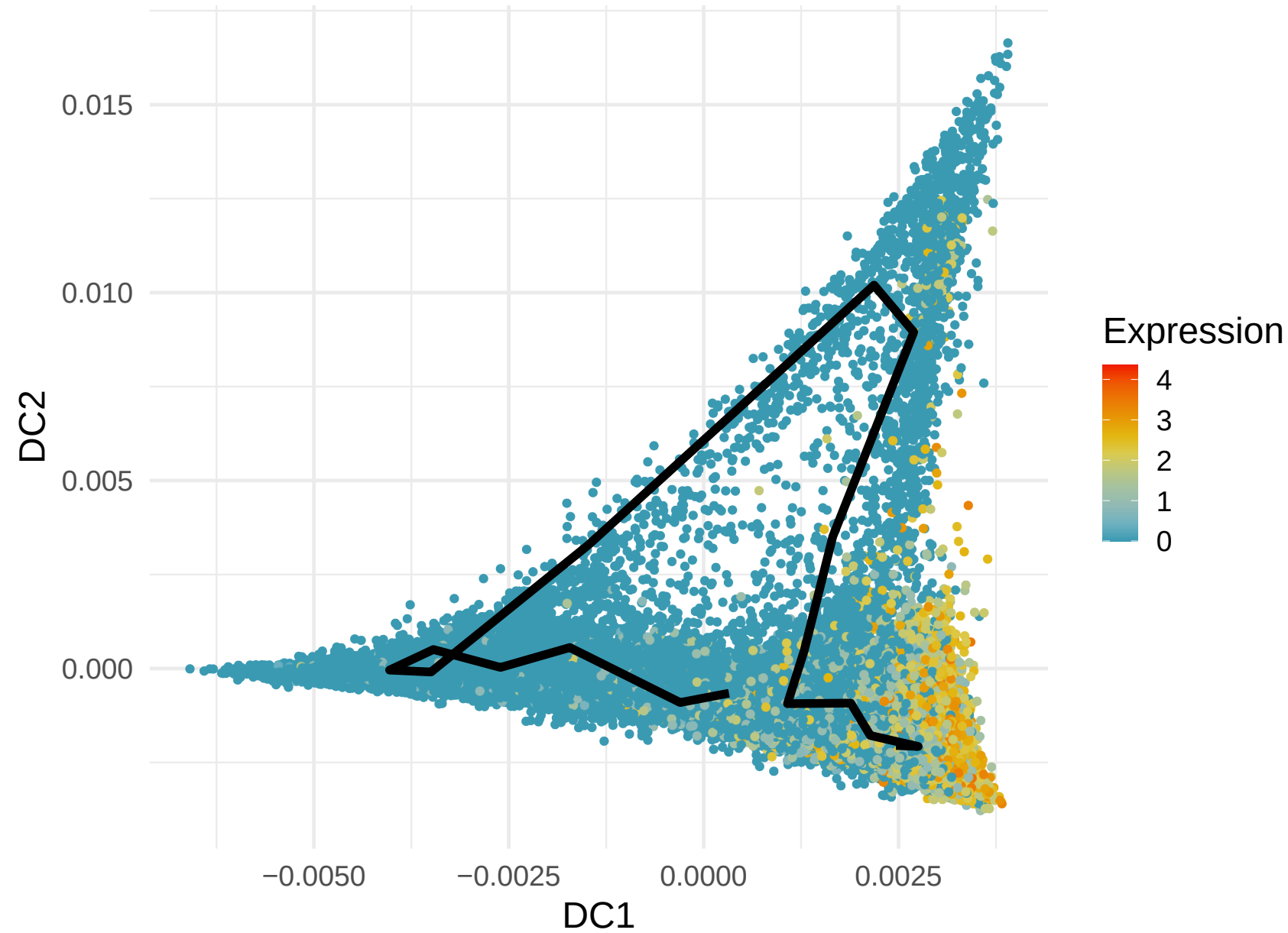
FGFBP2 Expression along Lineage 1 (R= 0.622)
