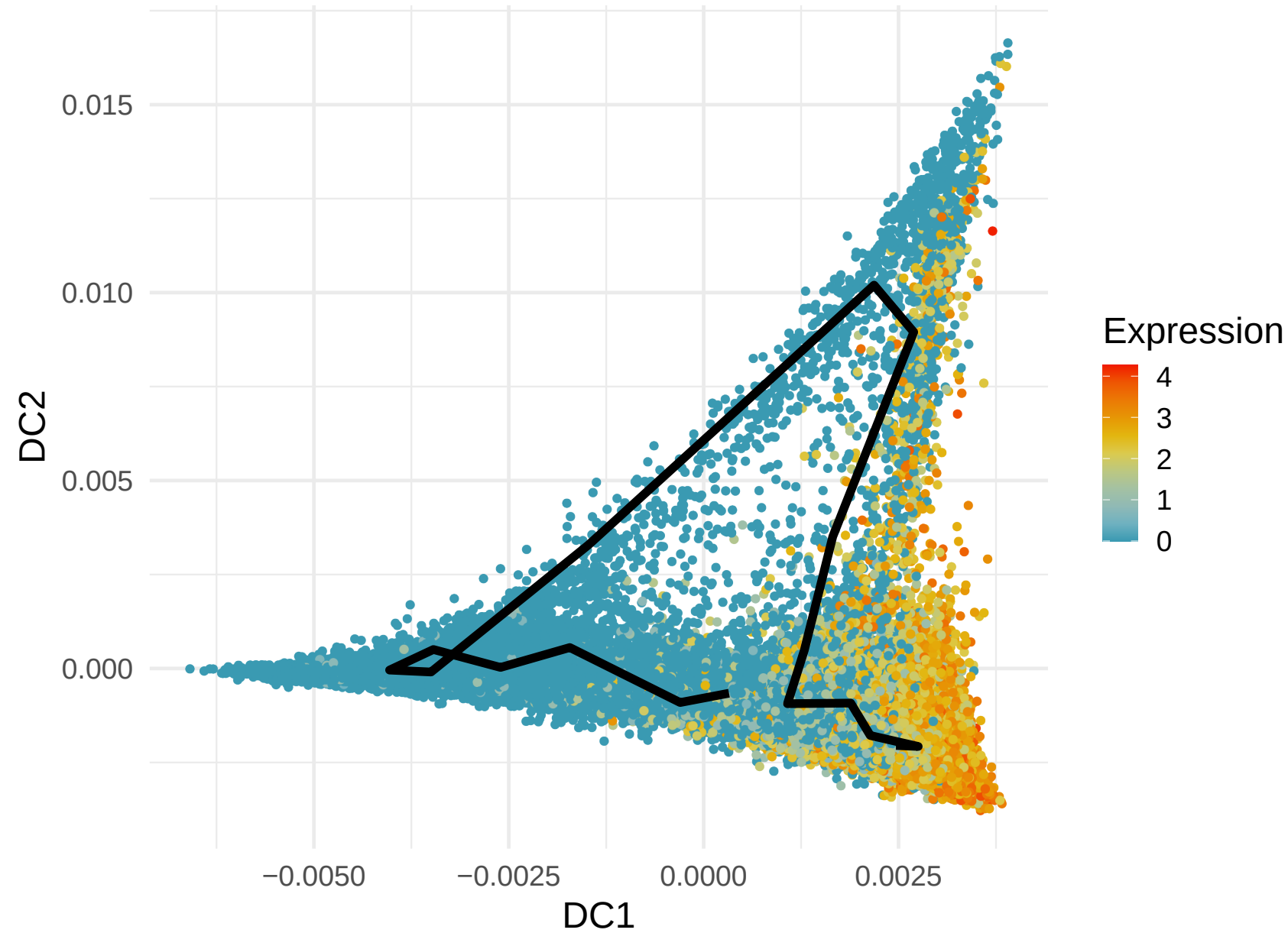
GZMH Expression along Lineage 1 (R= 0.709)
