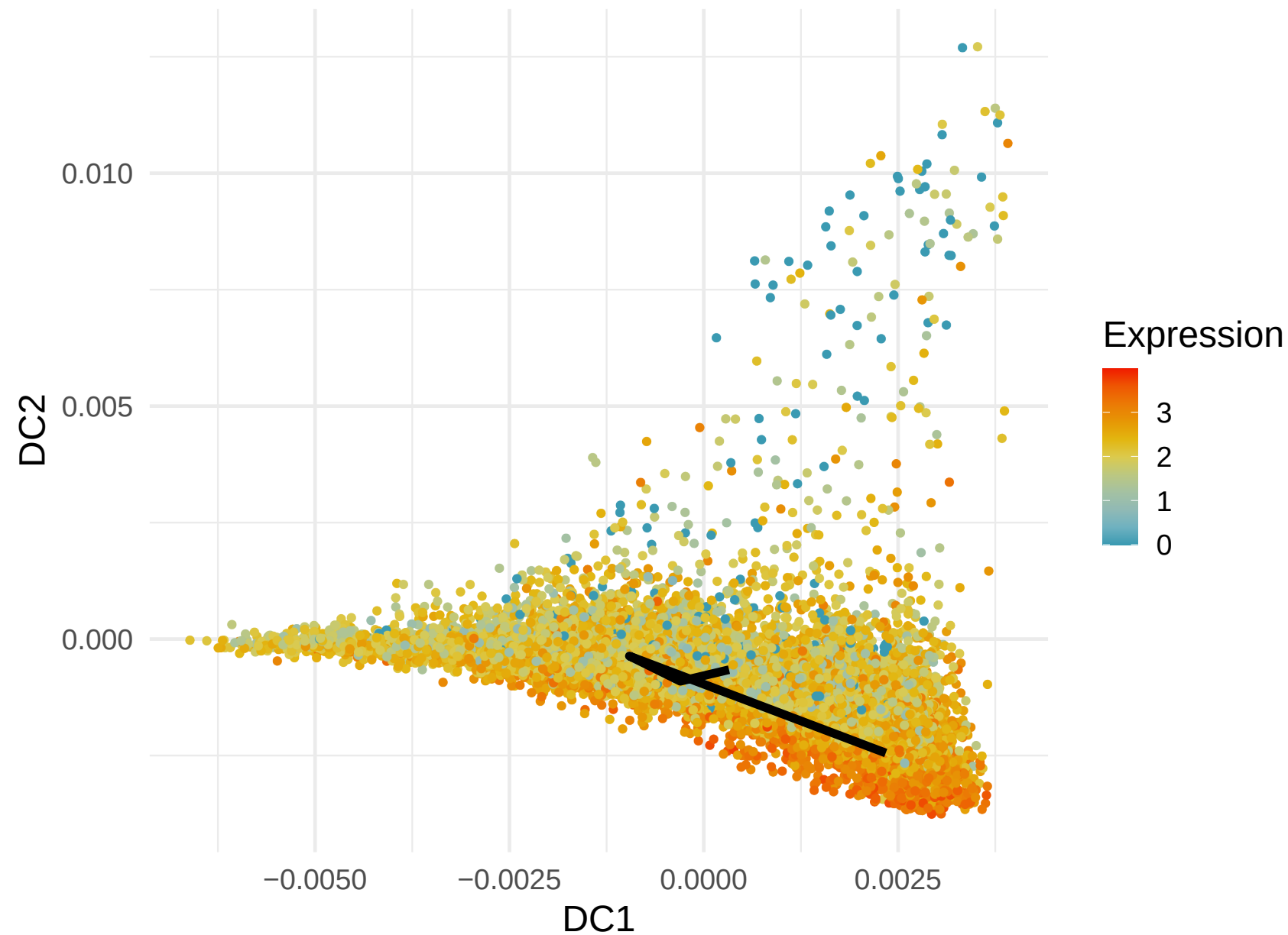
CFL1 Expression along Lineage 10 ( R = 0.373 )
