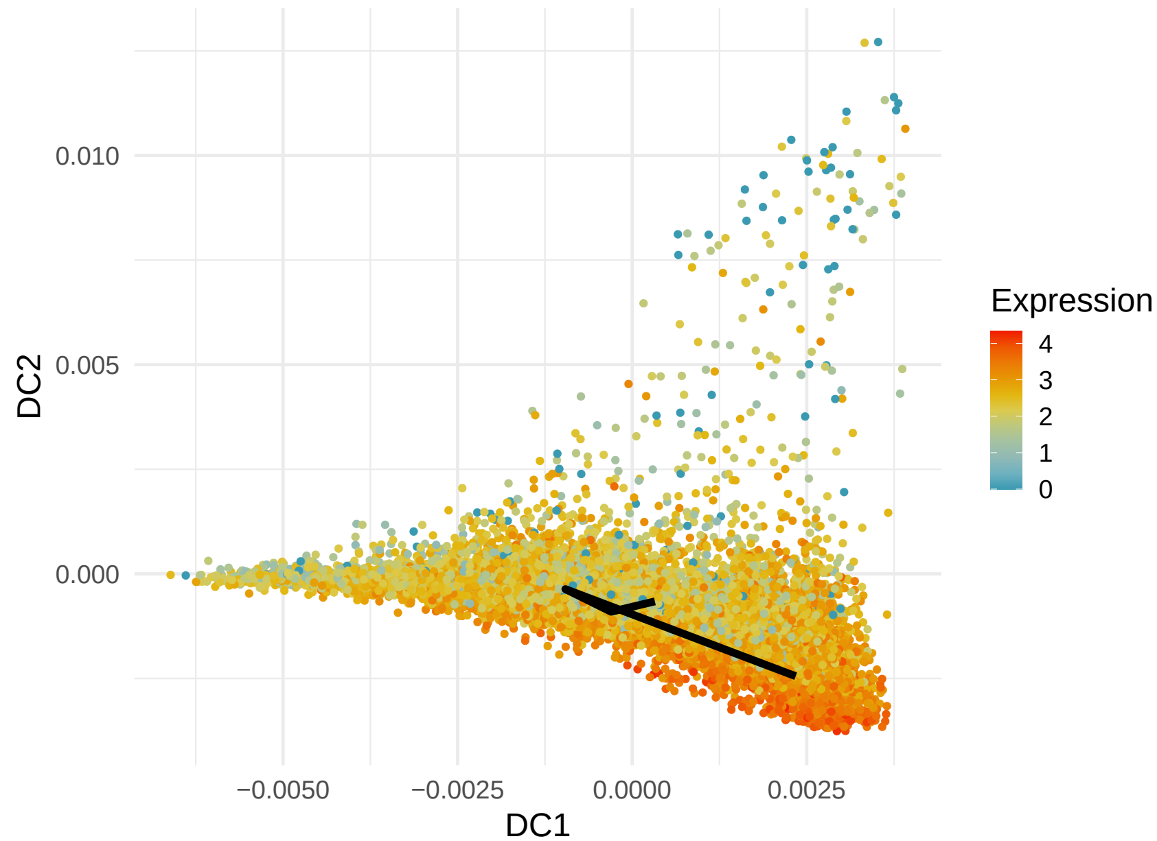
PFN1 Expression along Lineage 10 ( R = 0.437 )
