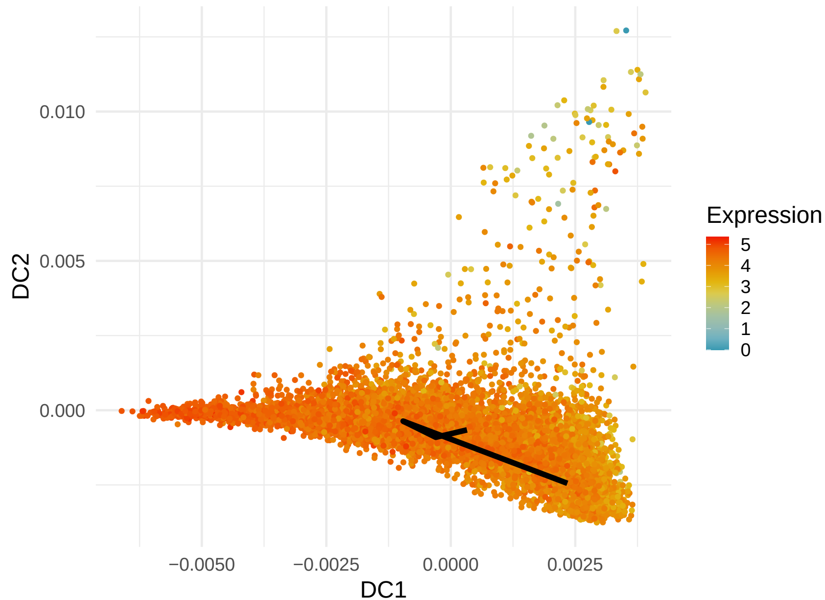
RPL13 Expression along Lineage 10 ( R = -0.309 )
