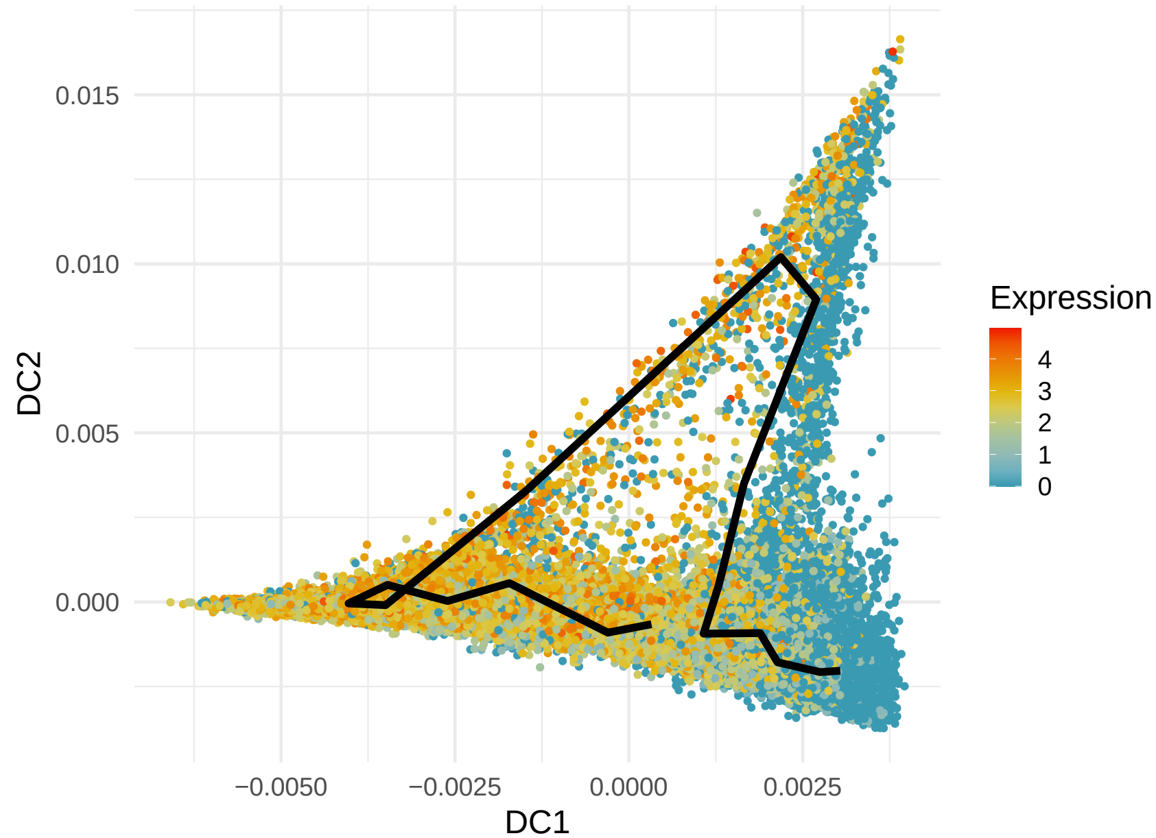
IL7R Expression along Lineage 2 ( R = -0.527 )
