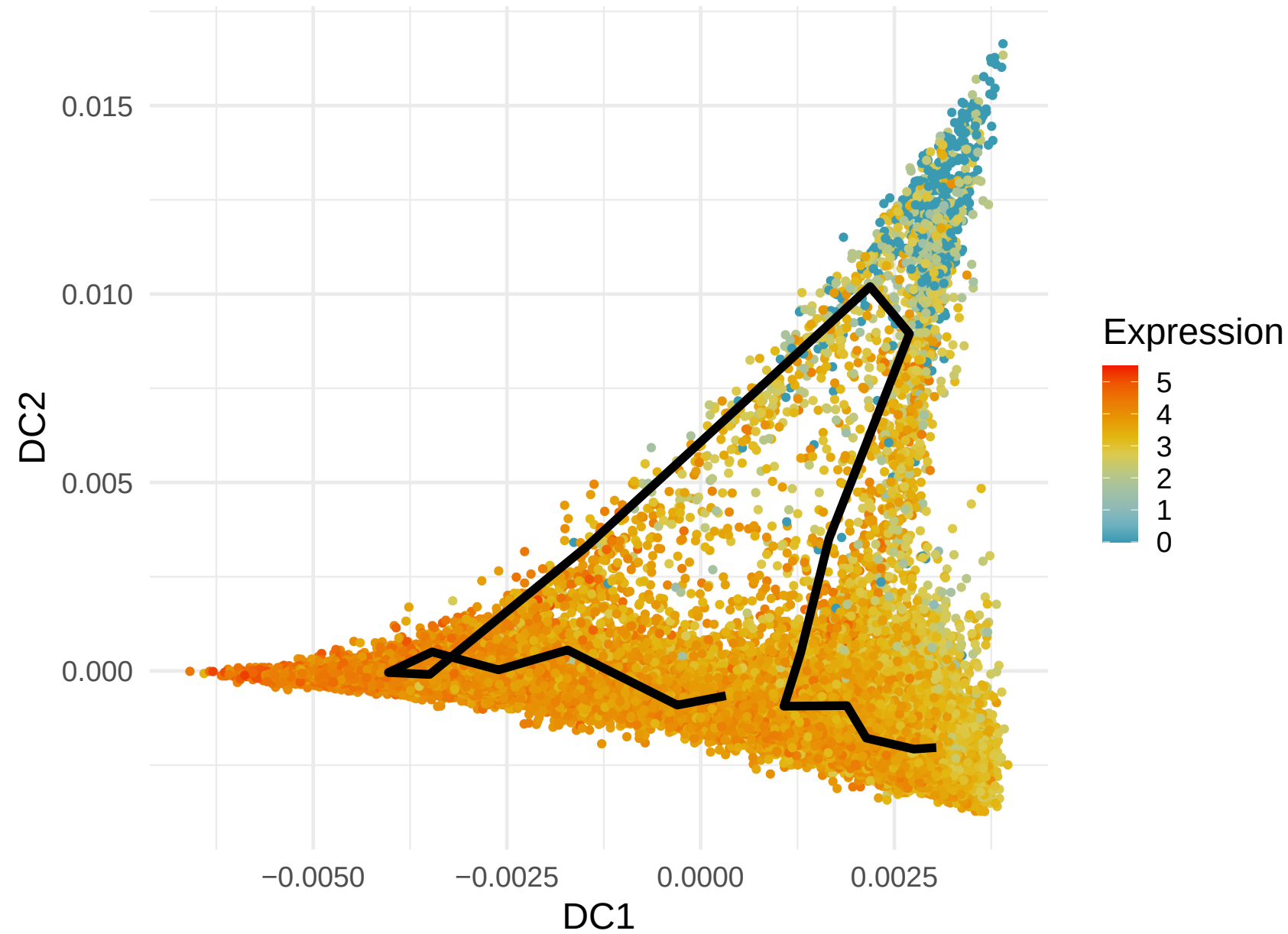
RPL39 Expression along Lineage 2 ( R = -0.32 )
