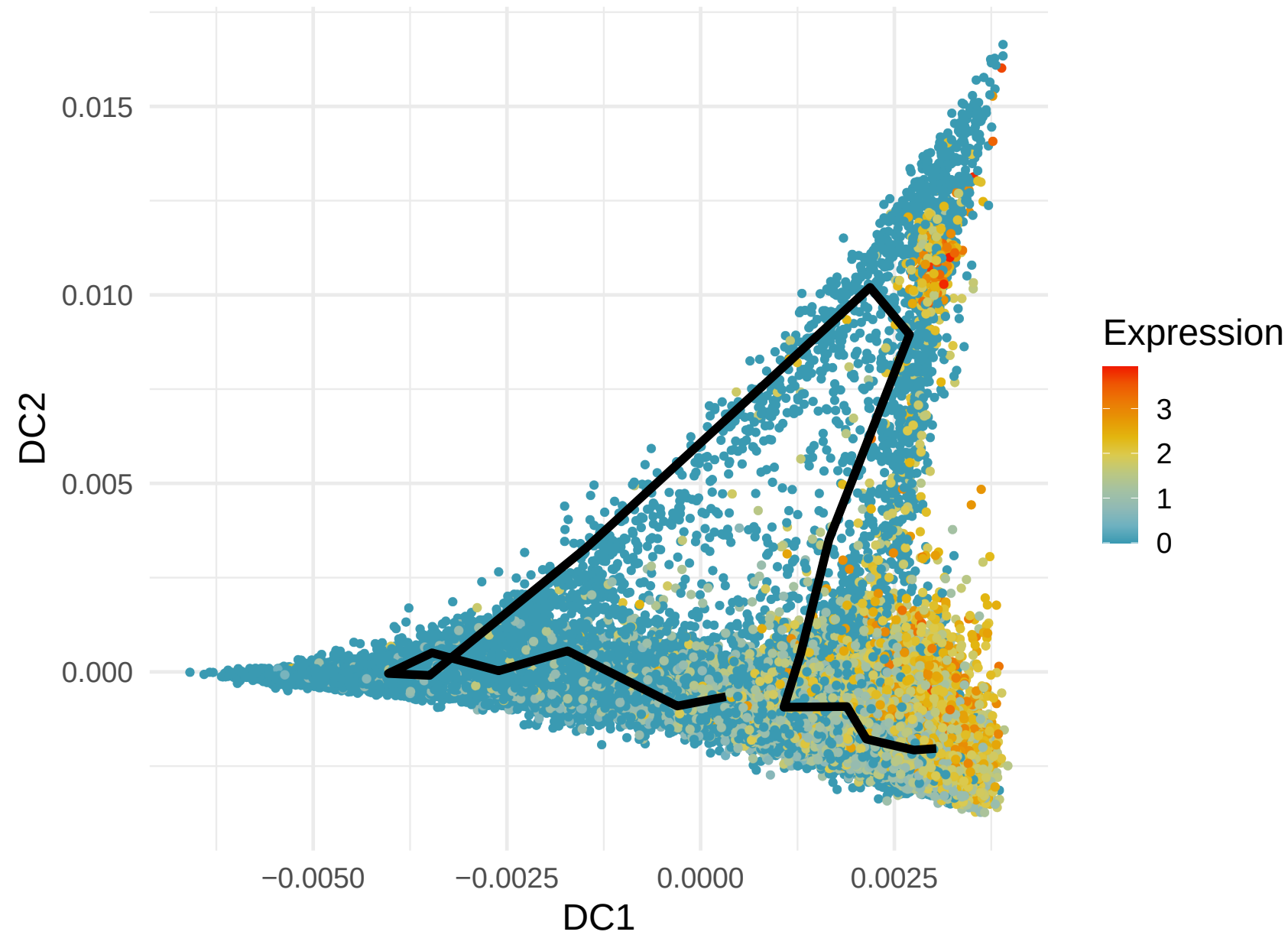
ZEB2 Expression along Lineage 2 ( R = 0.502 )
