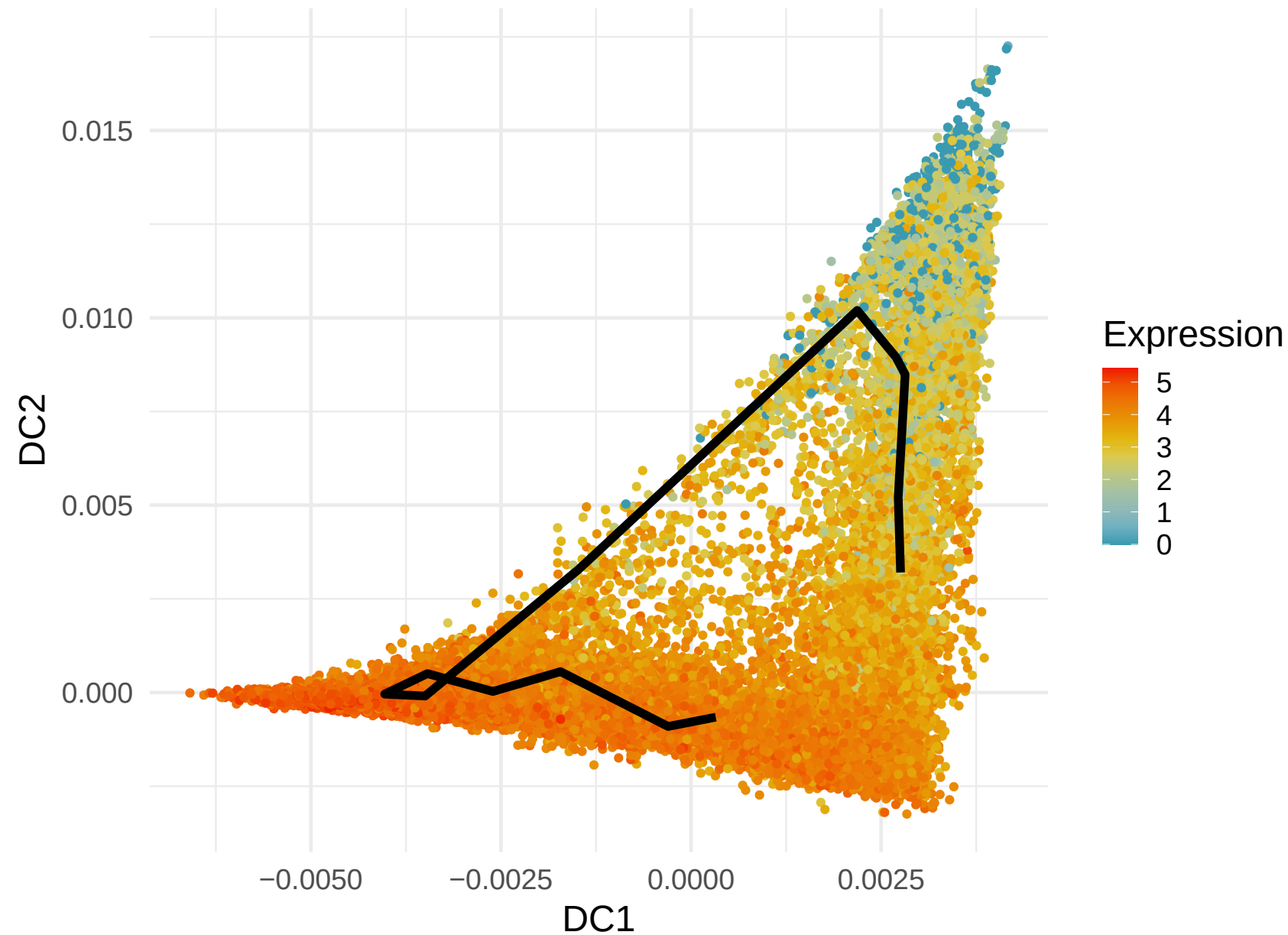
RPL10 Expression along Lineage 4 ( R = -0.393 )
