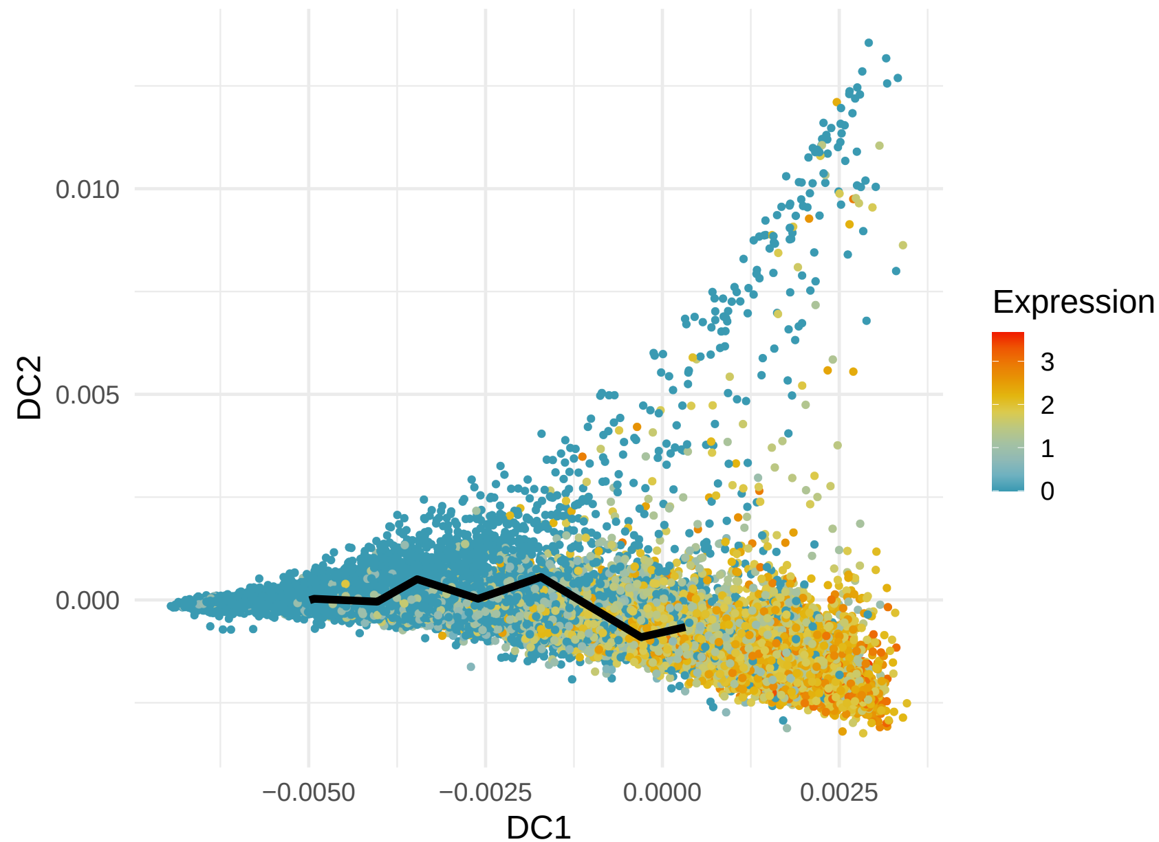
CST7 Expression along Lineage 6 ( R = -0.53 )
