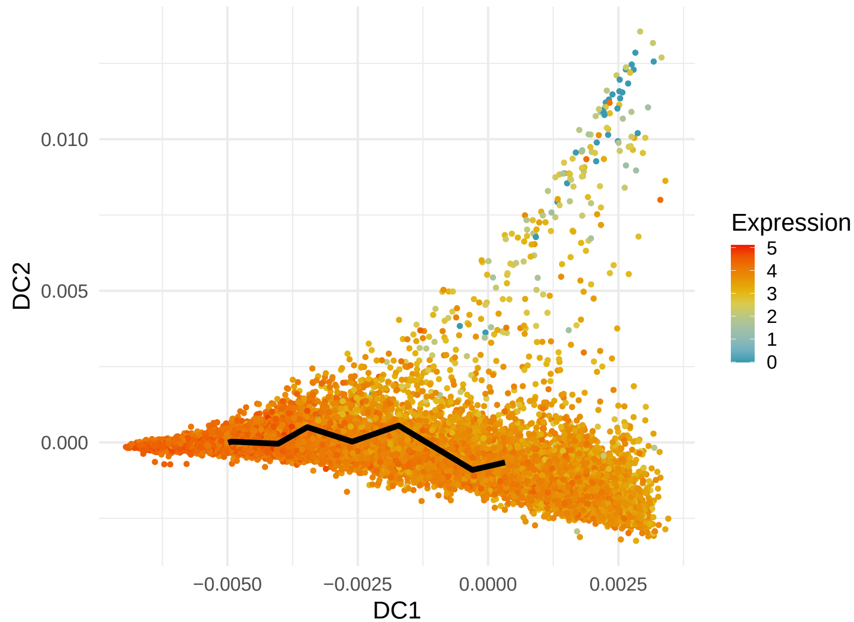
RPS23 Expression along Lineage 6 ( R = 0.513 )
