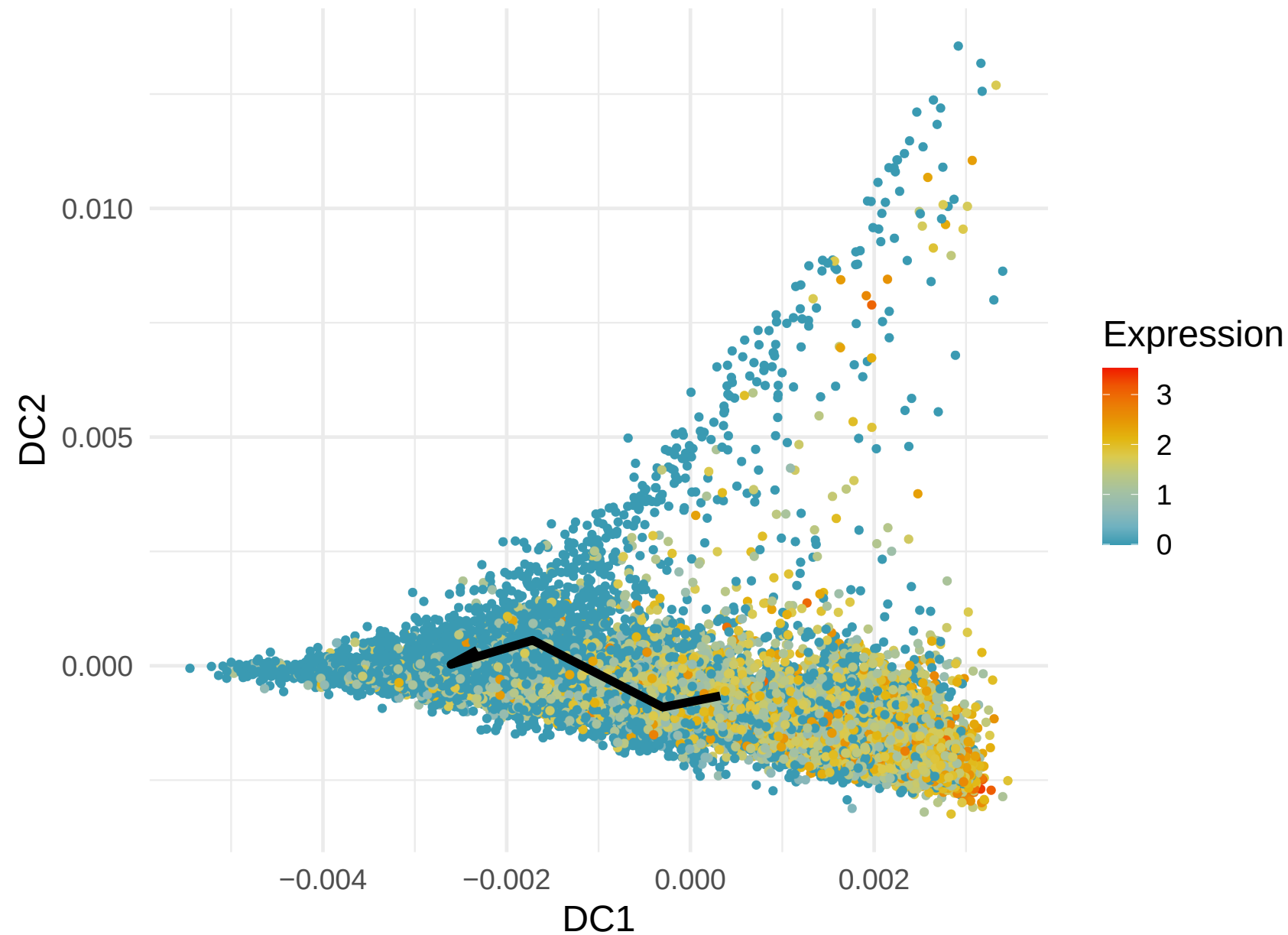
CTSW Expression along Lineage 8 ( R = -0.34 )
