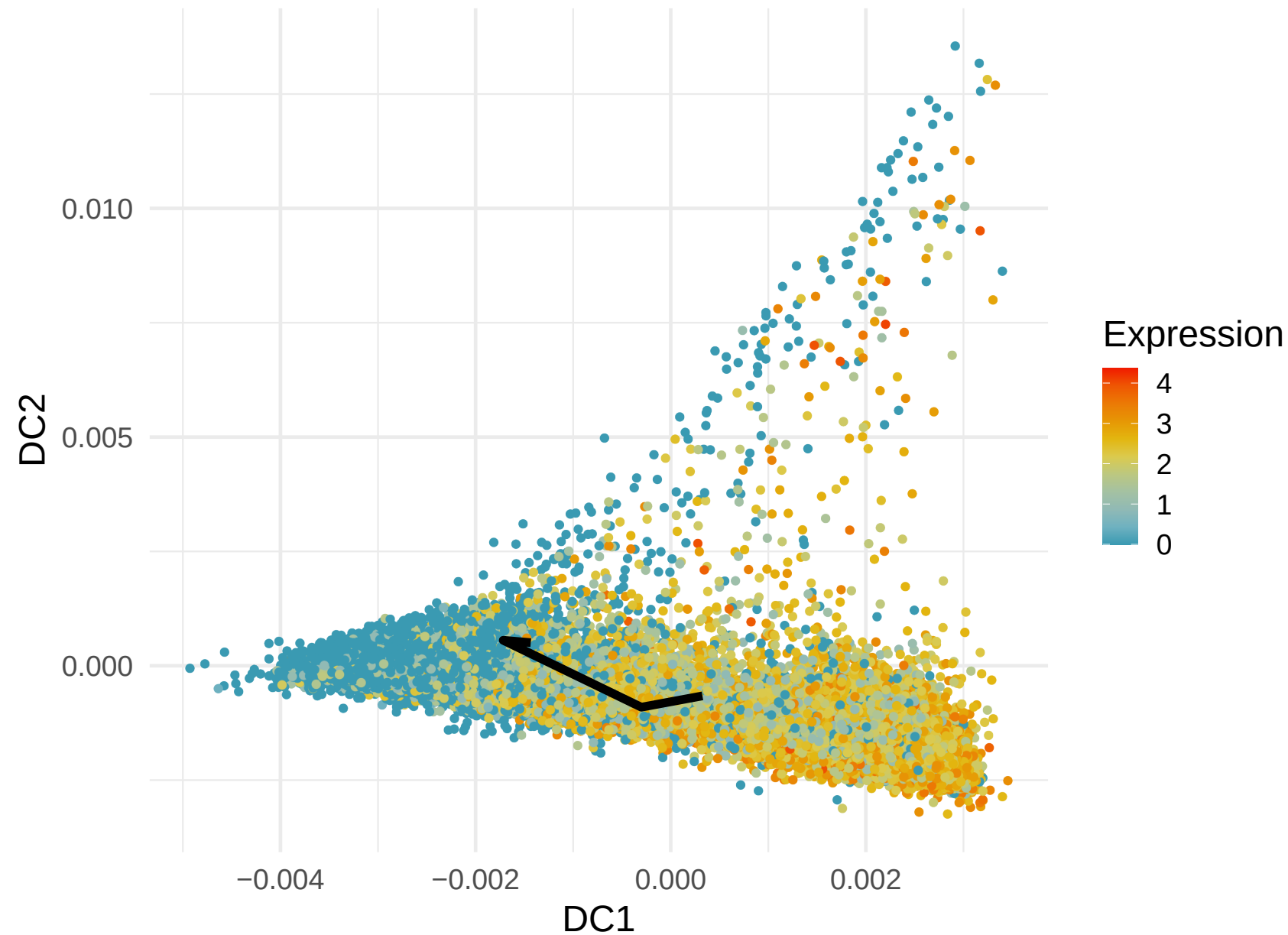
GZMA Expression along Lineage 9 ( R = -0.474 )
