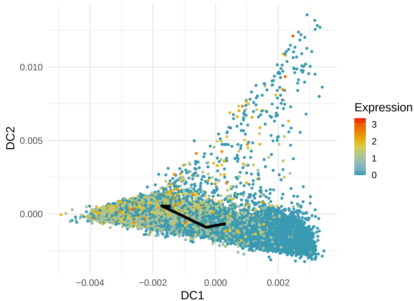
RCAN3 Expression along Lineage 9 ( R = 0.279 )
