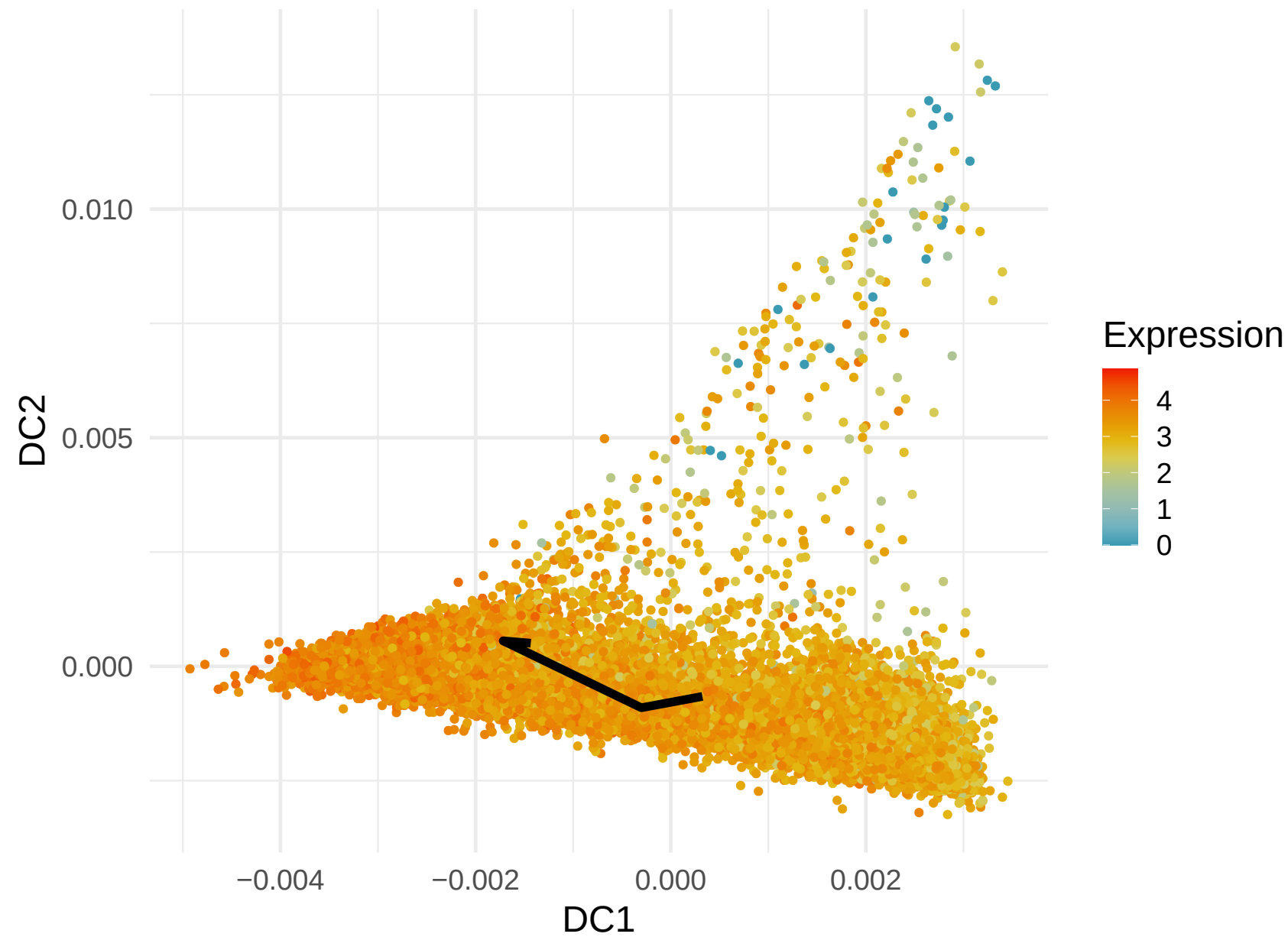
RPL36 Expression along Lineage 9 ( R = 0.336 )
